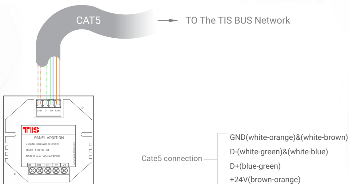
▲ Figure 5: ADD-2DL-IRE & Bus Connection Color Coding
