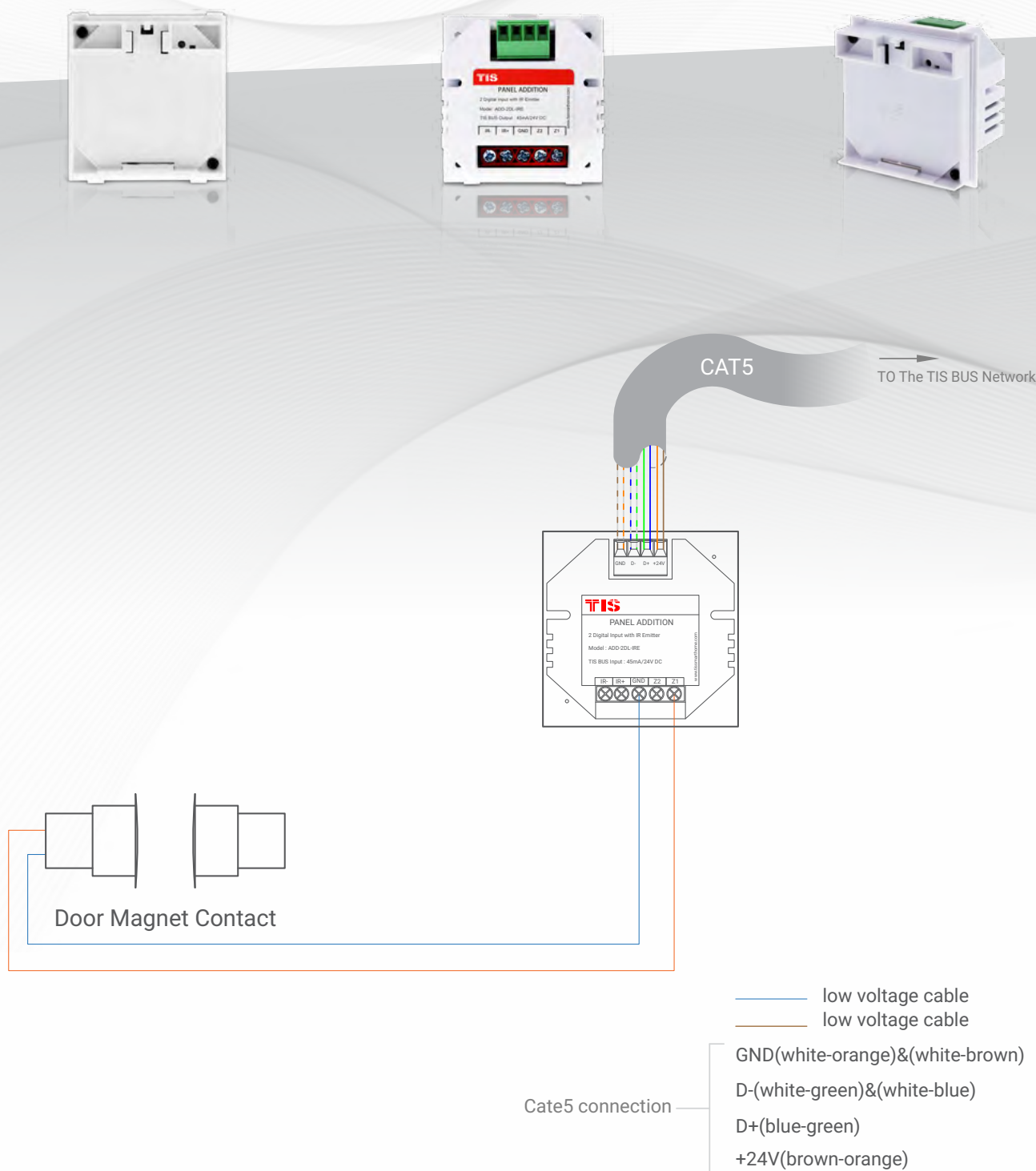
▲ Figure 1: ADD-2DL-IRE & Magnetic Door Contact Connection Diagram
