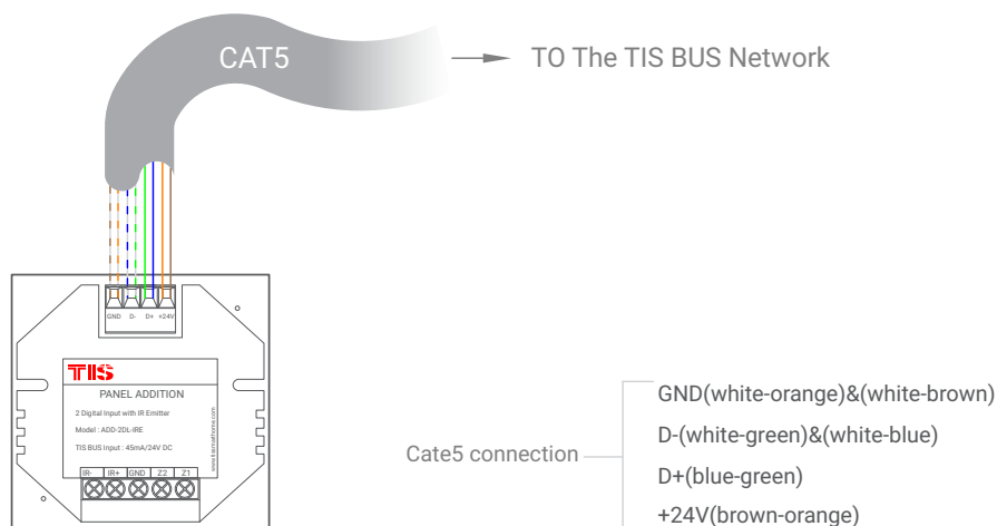
▲ Figure 5: Bus Connection Color Coding
