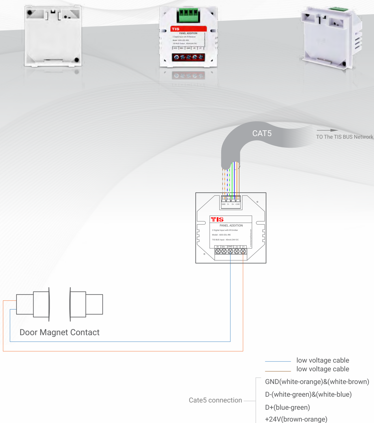
▲ Figure 1: ADD-2DL-IRR & Magnetic Door Contact Connection Diagram
