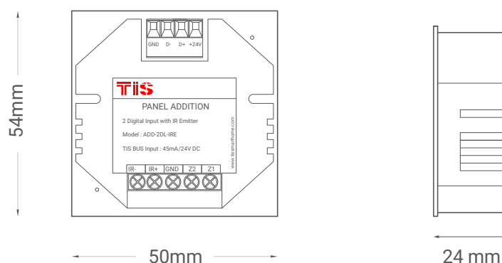
▲ Figure 6: Module Dimensions
