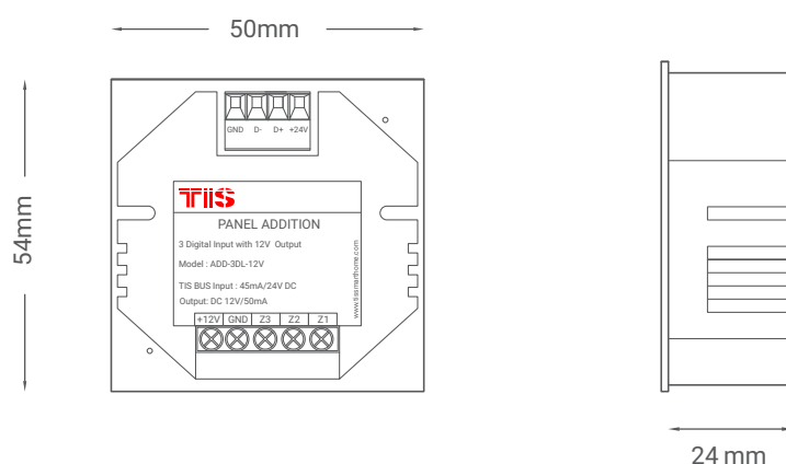
▲ Figure 5: Module Dimensions
