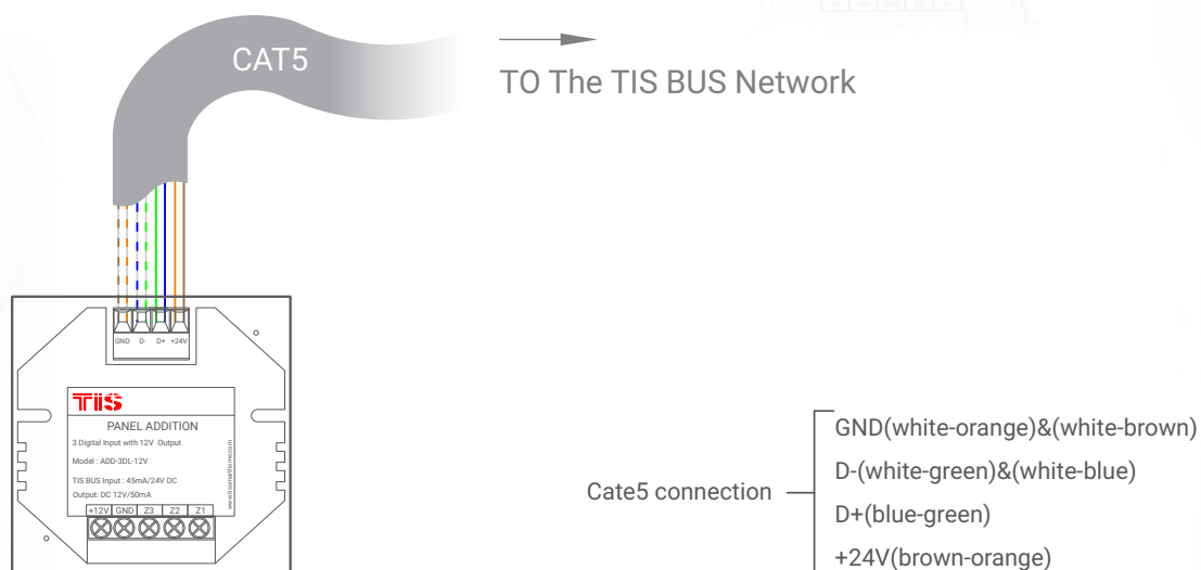
▲ Figure 4: Bus Connection Color Coding
