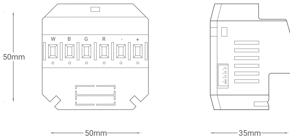
▲ Figure 5: Module Dimensions
