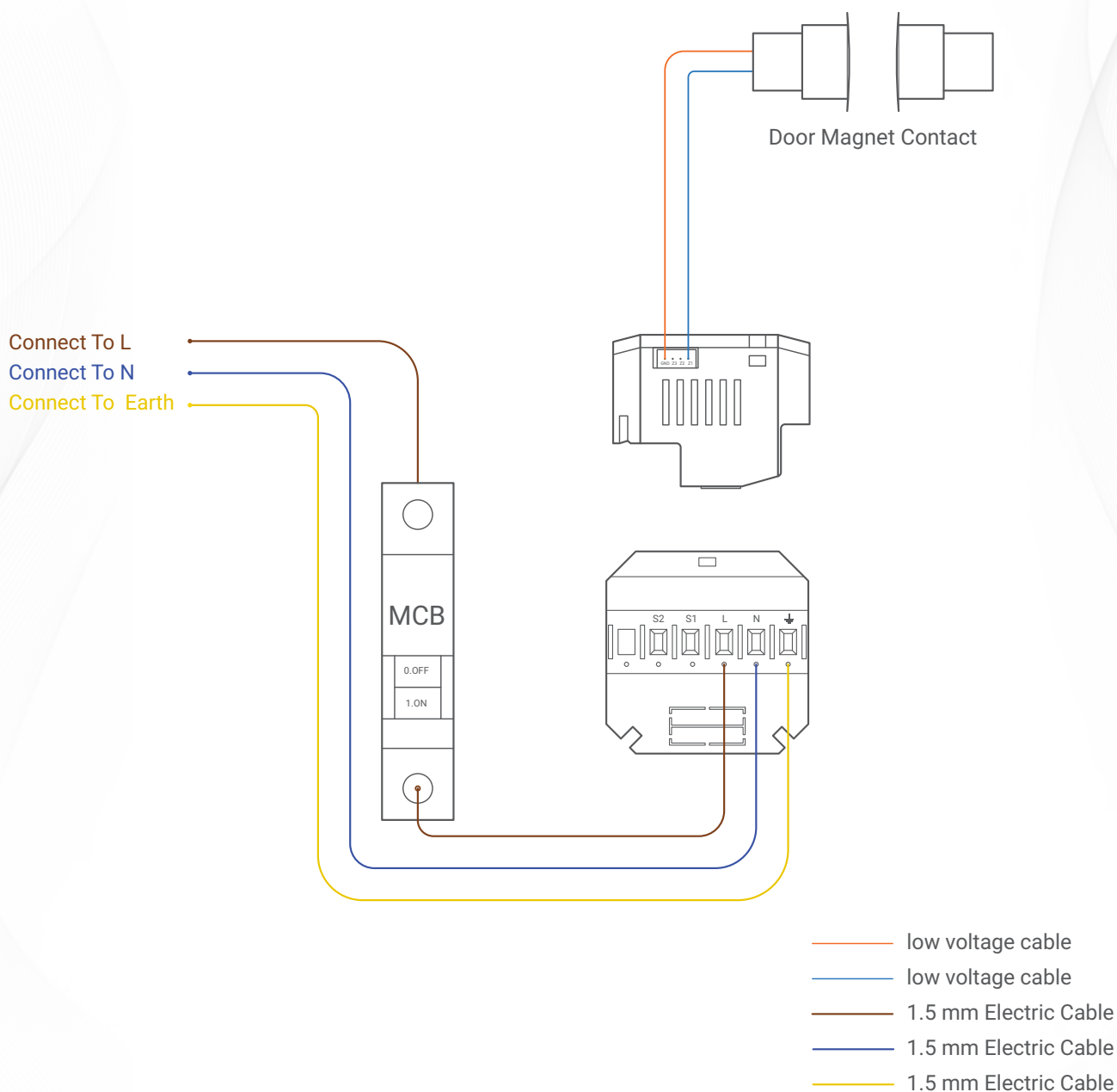
▲ Figure 3: Magnetic Door Contact Connection Diagram
