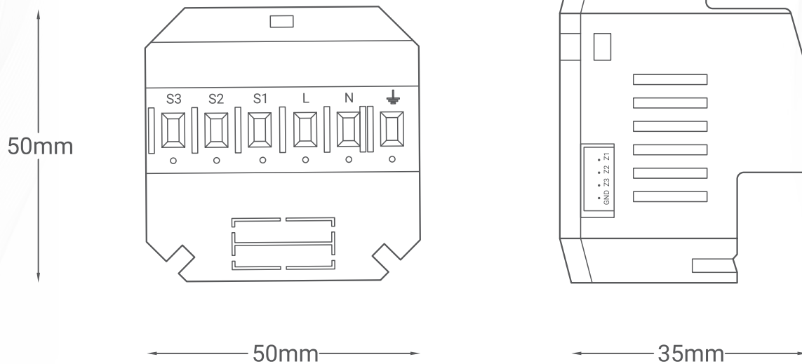
▲ Figure 8: Module Dimensions
