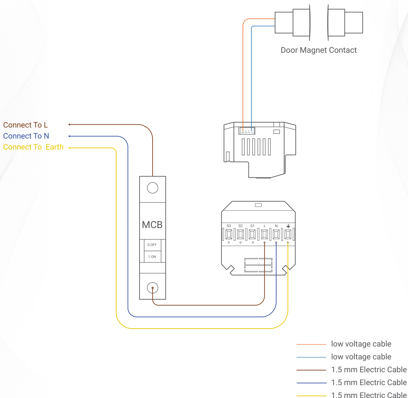
▲ Figure 5: Magnetic Door Contact Connection Diagram
