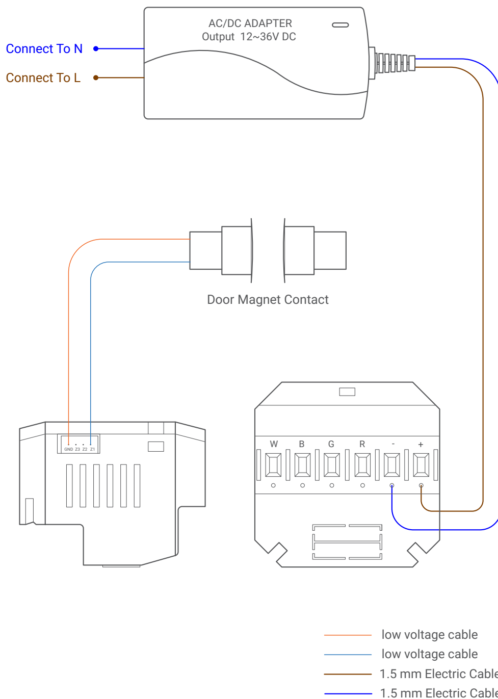
▲ Figure 2: Magnetic Door Contact Connection Diagram
