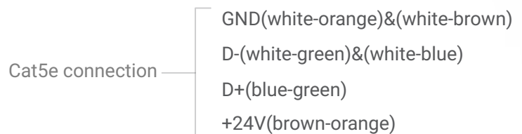
▲ Figure 2: BUS Connection Color Coding
