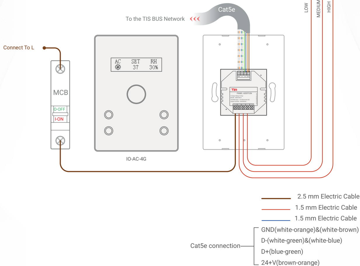
▲ Figure 2: IO-AC-4G & ADD-3R-5A & High/Med/Low FCU Unit Connection Diagram
