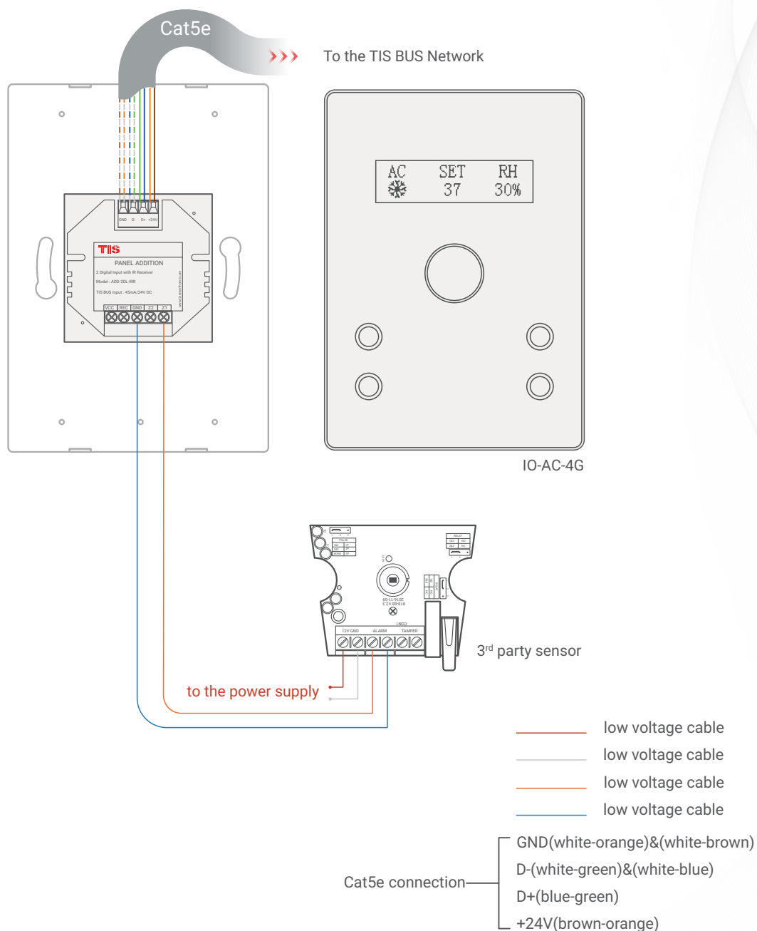
▲ Figure 10: IO-AC-4G & ADD-2DL-IRR & 3 rd Party Sensor Connection Diagram
