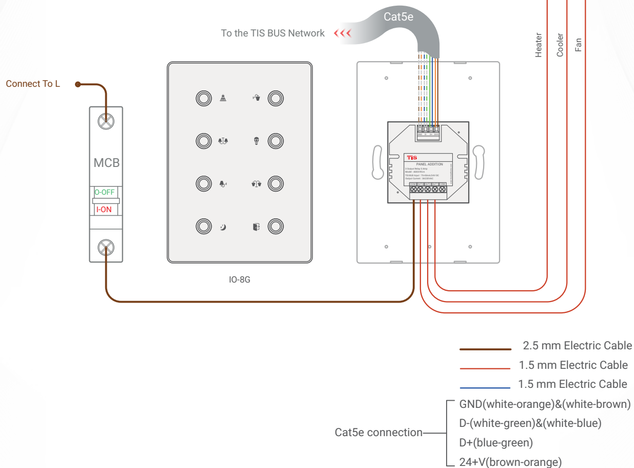
▲ Figure 3: IO-AC-4G & ADD-3R-5A & Heater/Cooler/Fan FCU Unit Connection Diagram
