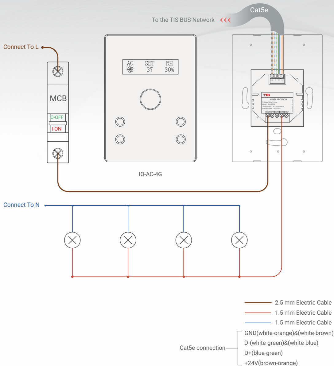
▲ Figure 1: IO-AC-4G & ADD-3R-5A & Lights Connection Diagram
