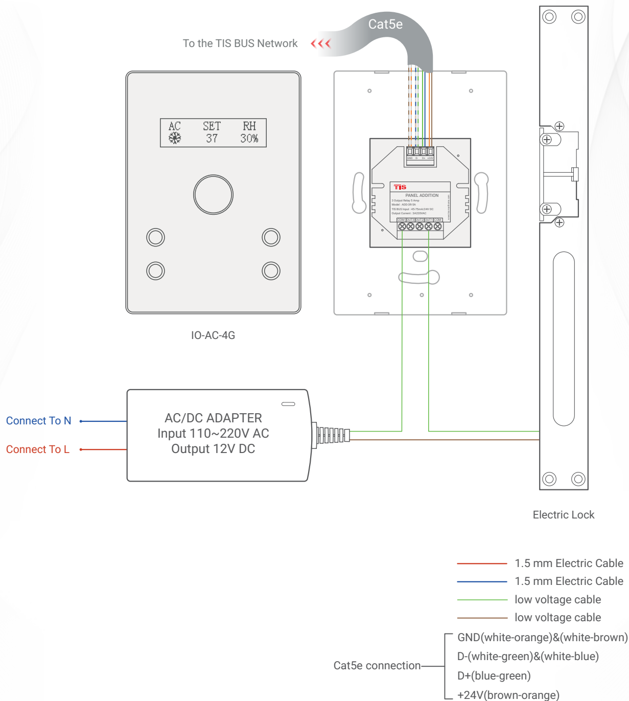
▲ Figure 5: IO-AC-4G & ADD-3R-5A & Electric Lock Connection Diagram
