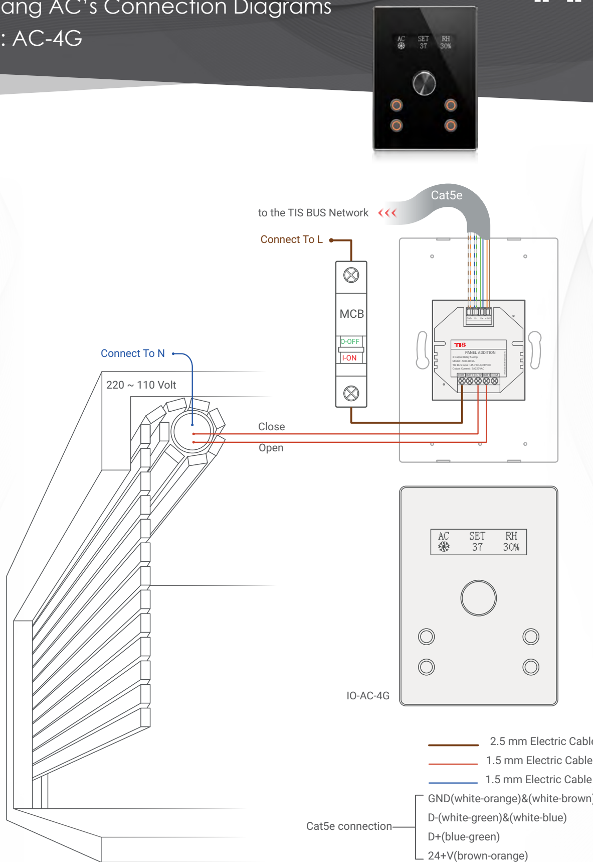
▲ Figure 4: IO-AC-4G & ADD-3R-5A & Motors Connection Diagram
