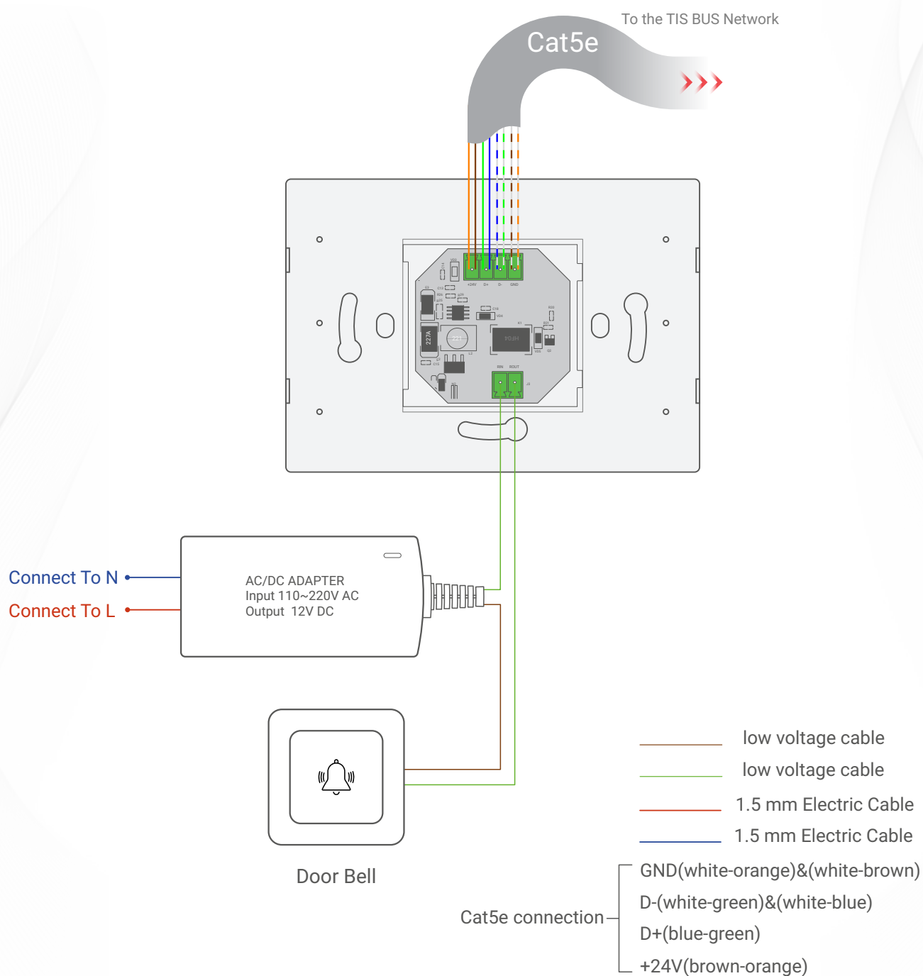
▲ Figure 3: IO-CARD-3SR & Door Bell Unit Connection Diagram
