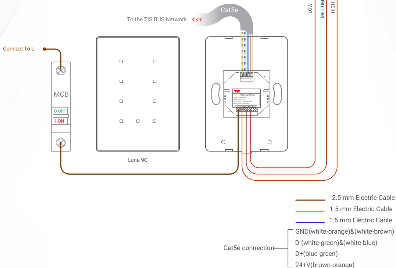
▲ Figure 3: ADD-3R-5A & Heater/Cooler/Fan FCU Unit Connection Diagram
