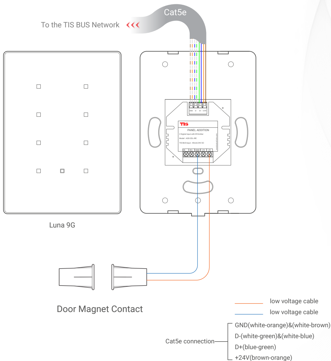
▲ Figure 12: Luna 9G & ADD-2DL-IRE Magnetic Door Contact Connection Diagram
