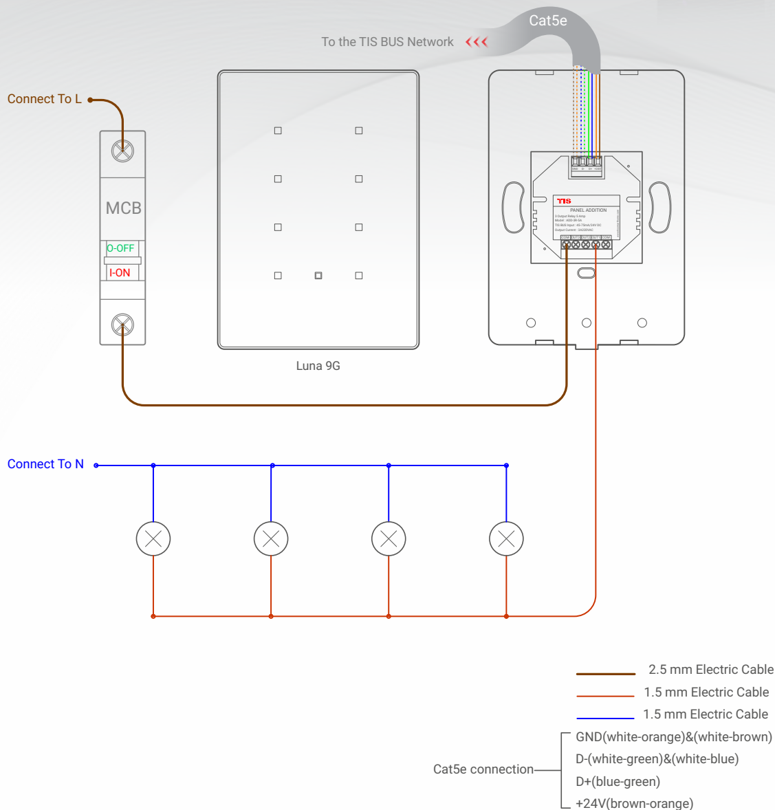
▲ Figure 1: Luna 9G & ADD-3R-5A Lights Connection Diagram
