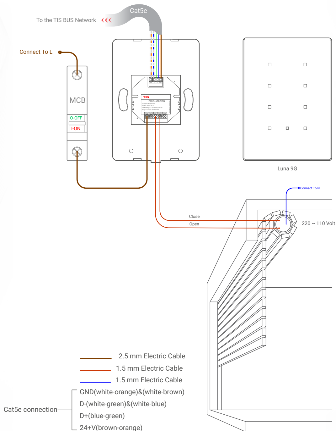
▲ Figure 4: Luna 9G & ADD-3R-5A Motors Connection Diagram
