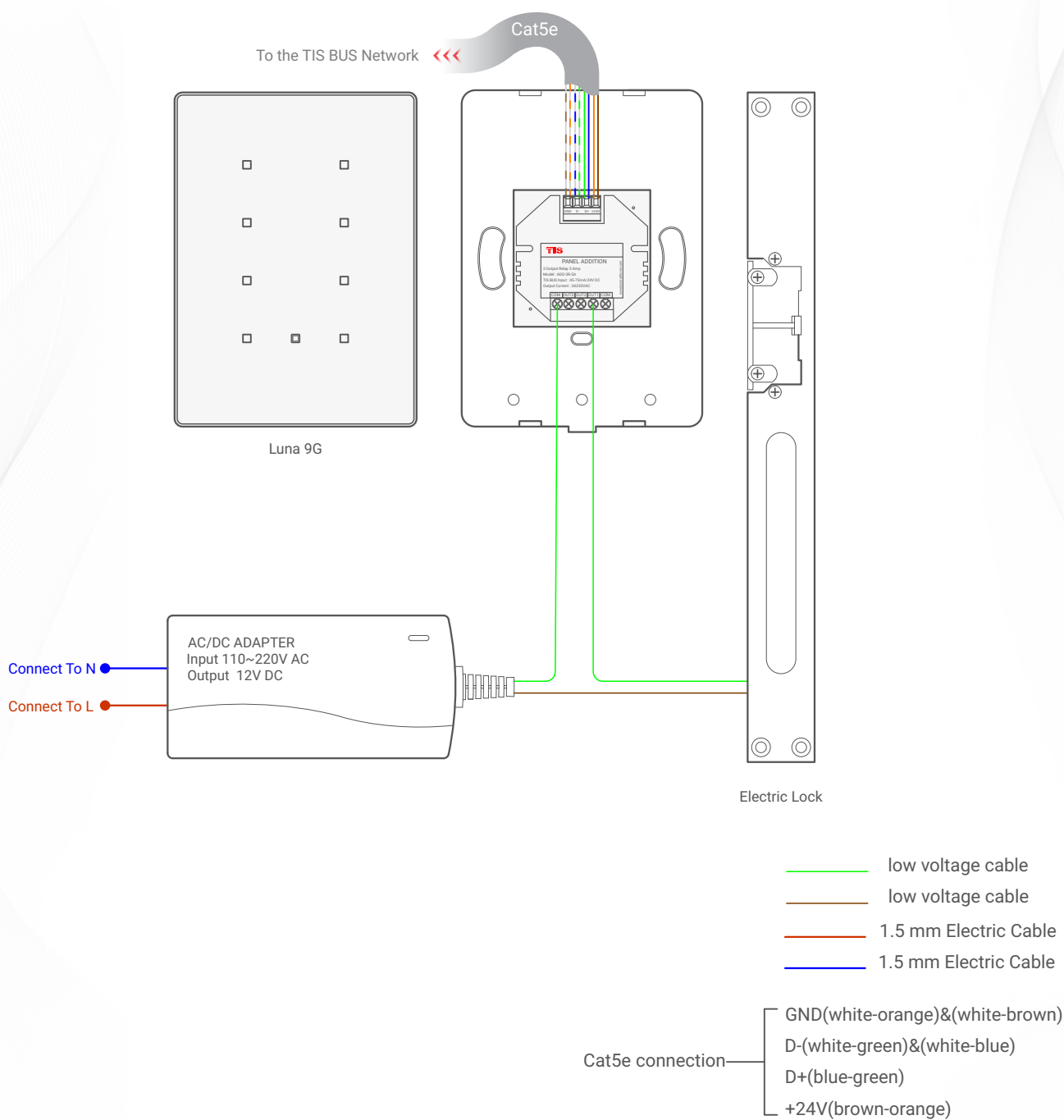
▲ Figure 5: Luna 9G & ADD-3R-5A Electric Lock Connection Diagram
