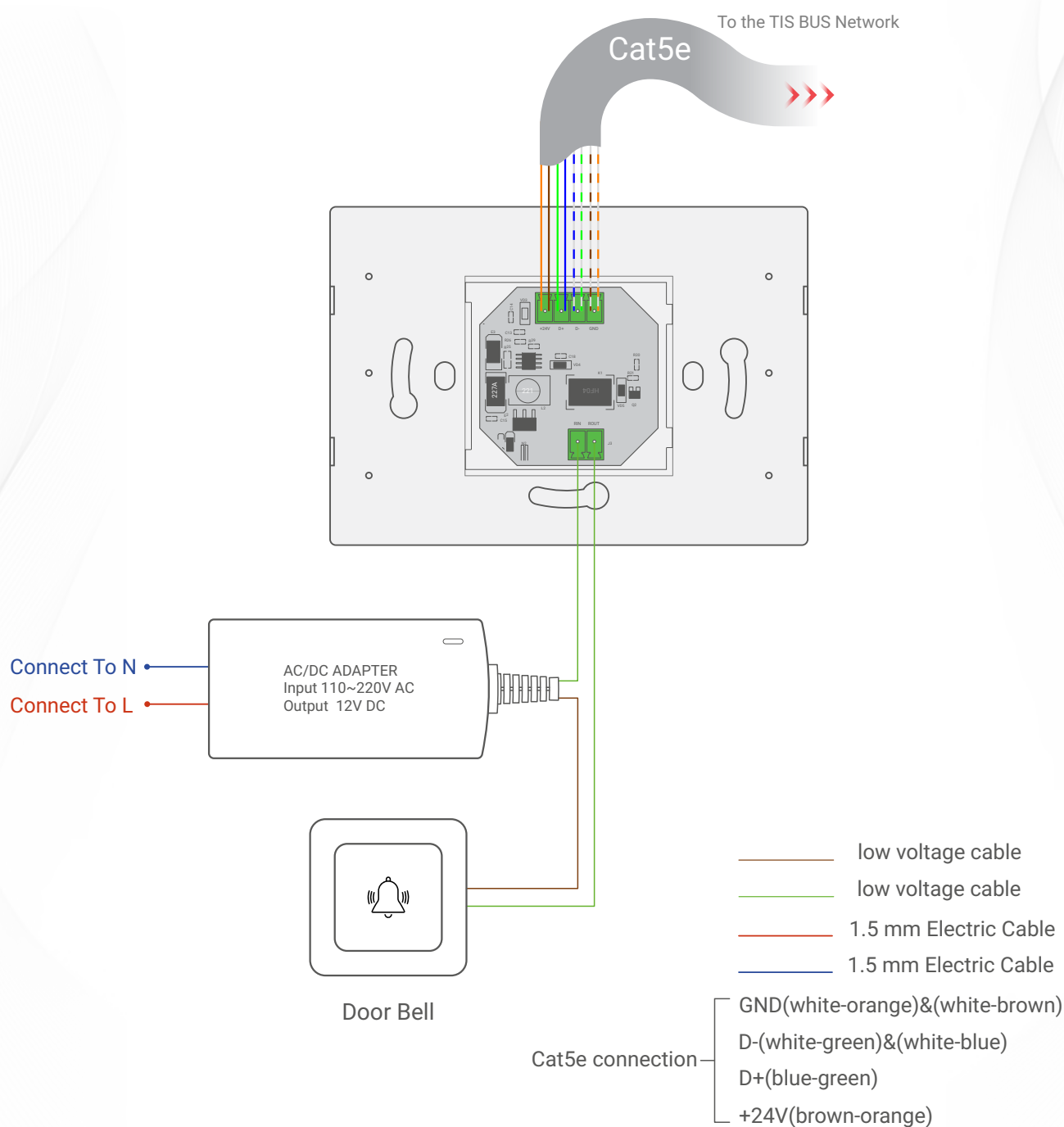
▲ Figure 2: LUNA-CARD&DoorBellUnitConnectionDiagram
