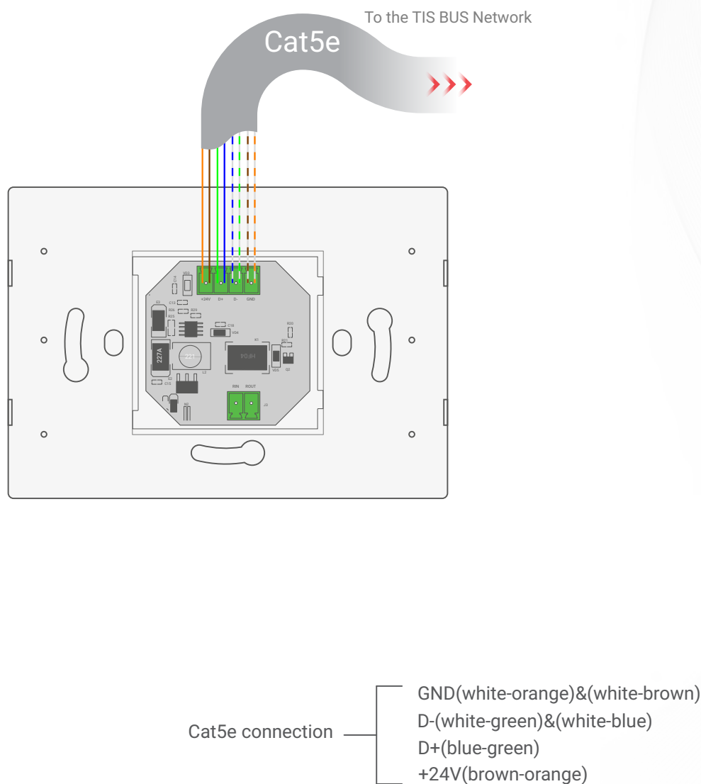
▲ Figure 3: LUNA-CARDModule'sBusConnectionColorCoding
