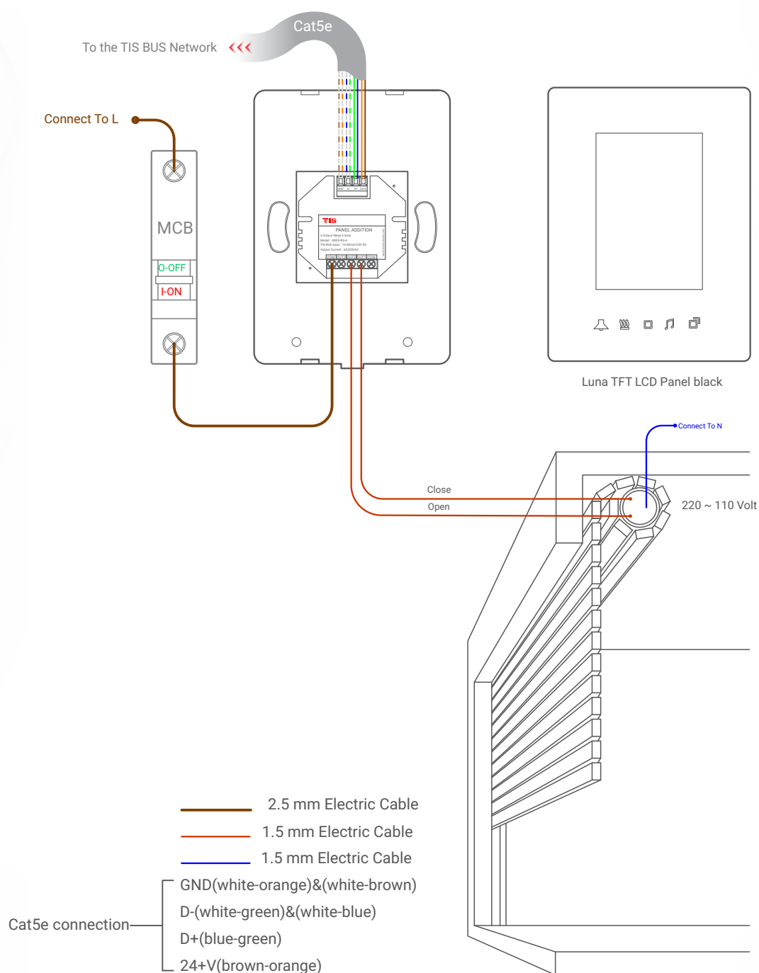
▲ Figure 3: Luna TFT & ADD-3R-5A Motors Connection Diagram
