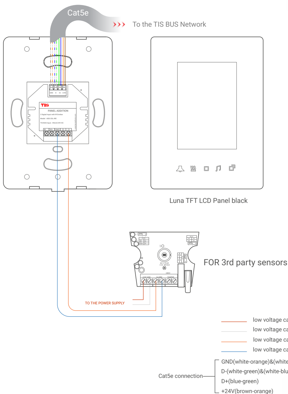
▲ Figure 12: Luna TFT & ADD-2DL-IRE 3 rd Party Sensor Connection Diagram
