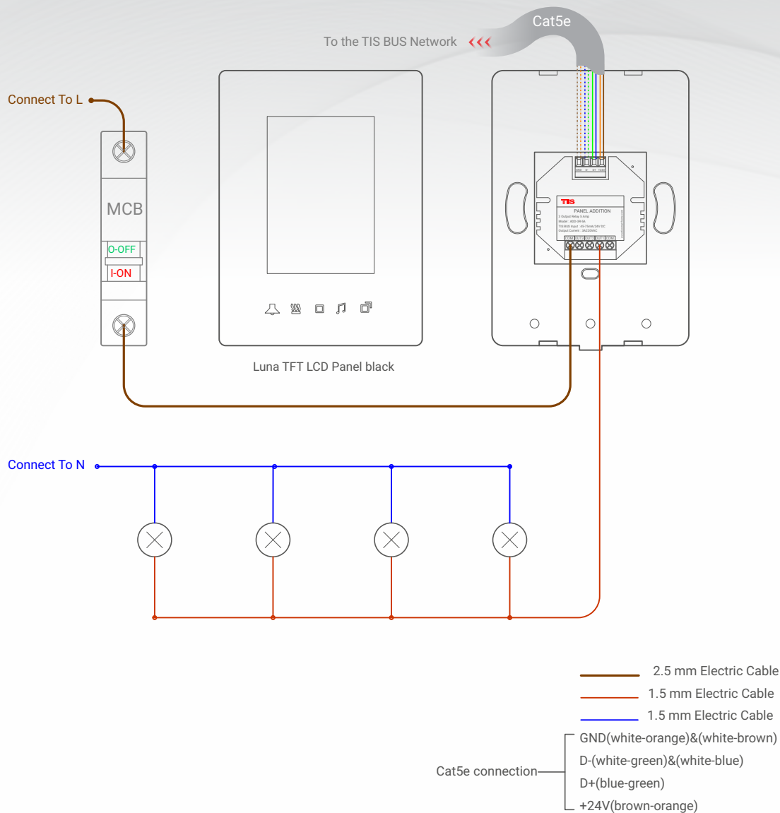
▲ Figure 1: Luna TFT & ADD-3R-5A Lights Connection Diagram
