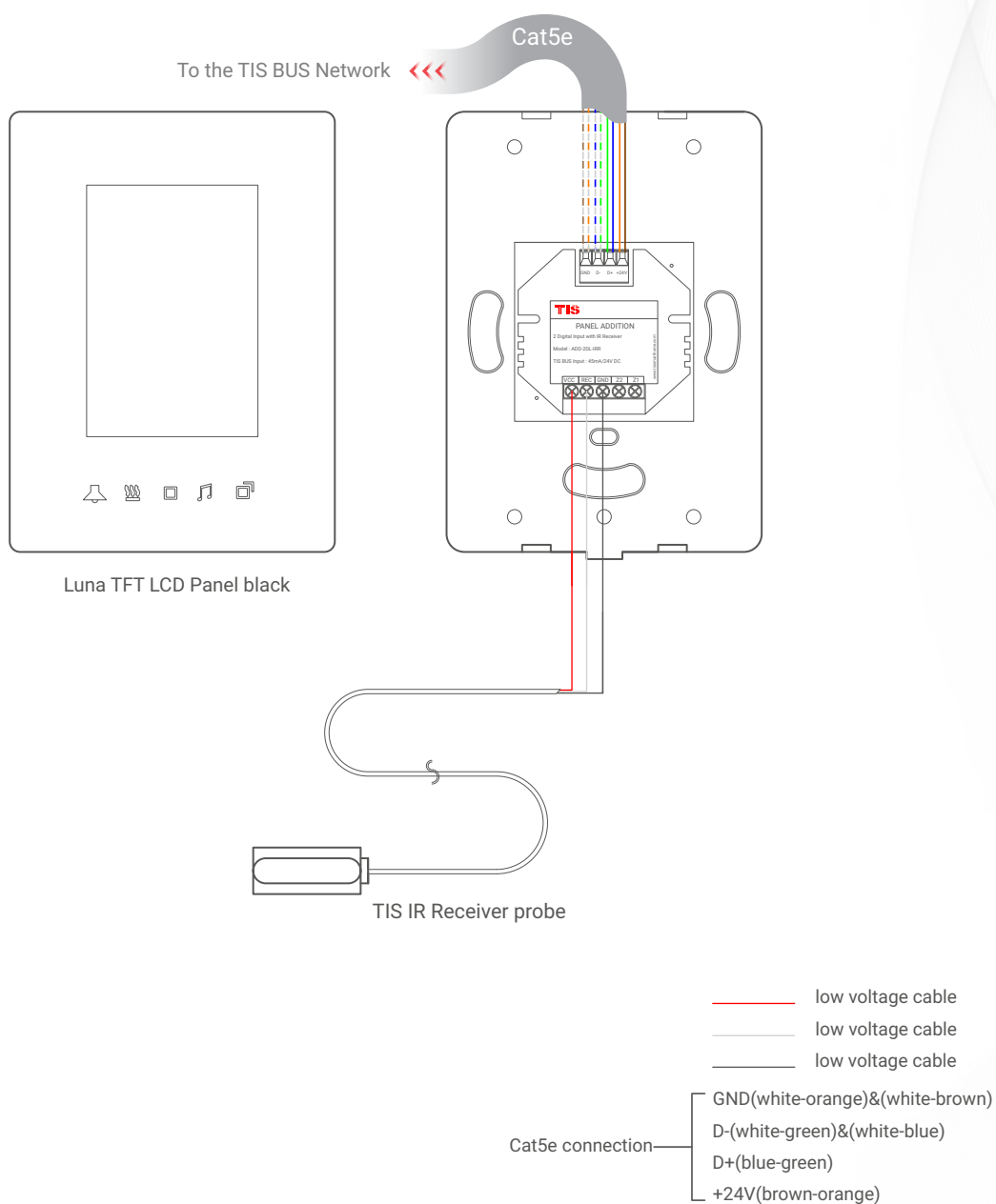
▲ Figure 7: Luna TFT & ADD-2DL-IRR Connection Diagram
