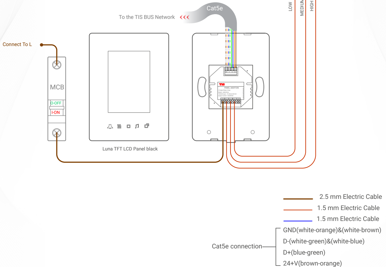
▲ Figure 2: Luna TFT & ADD-3R-5A FCU Connection Diagram
