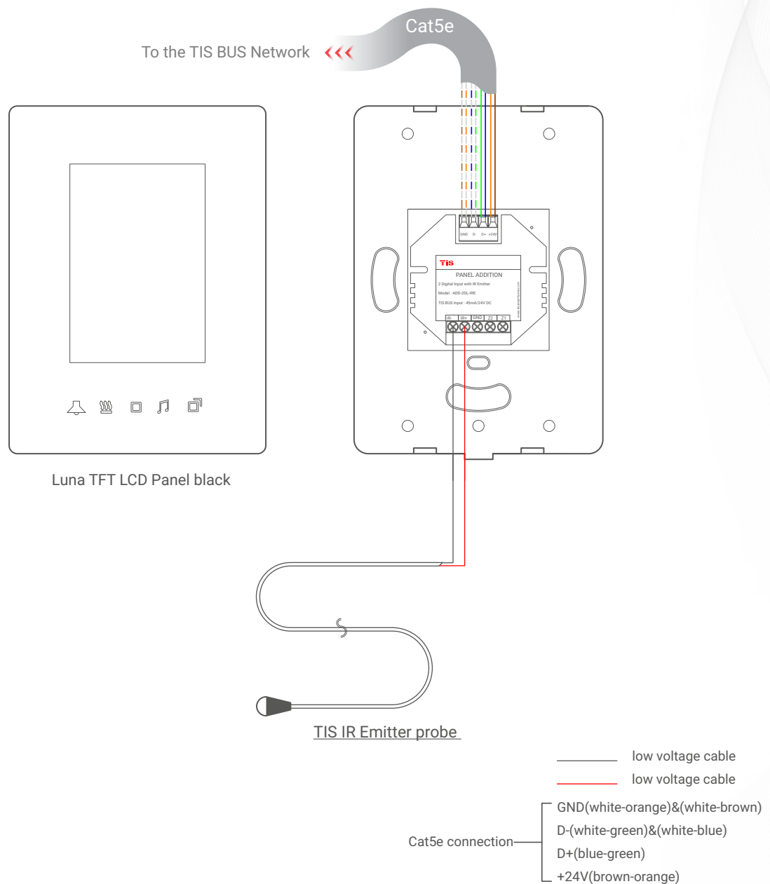
▲ Figure 10: Luna TFT & ADD-2DL-IRE Connection Diagram
