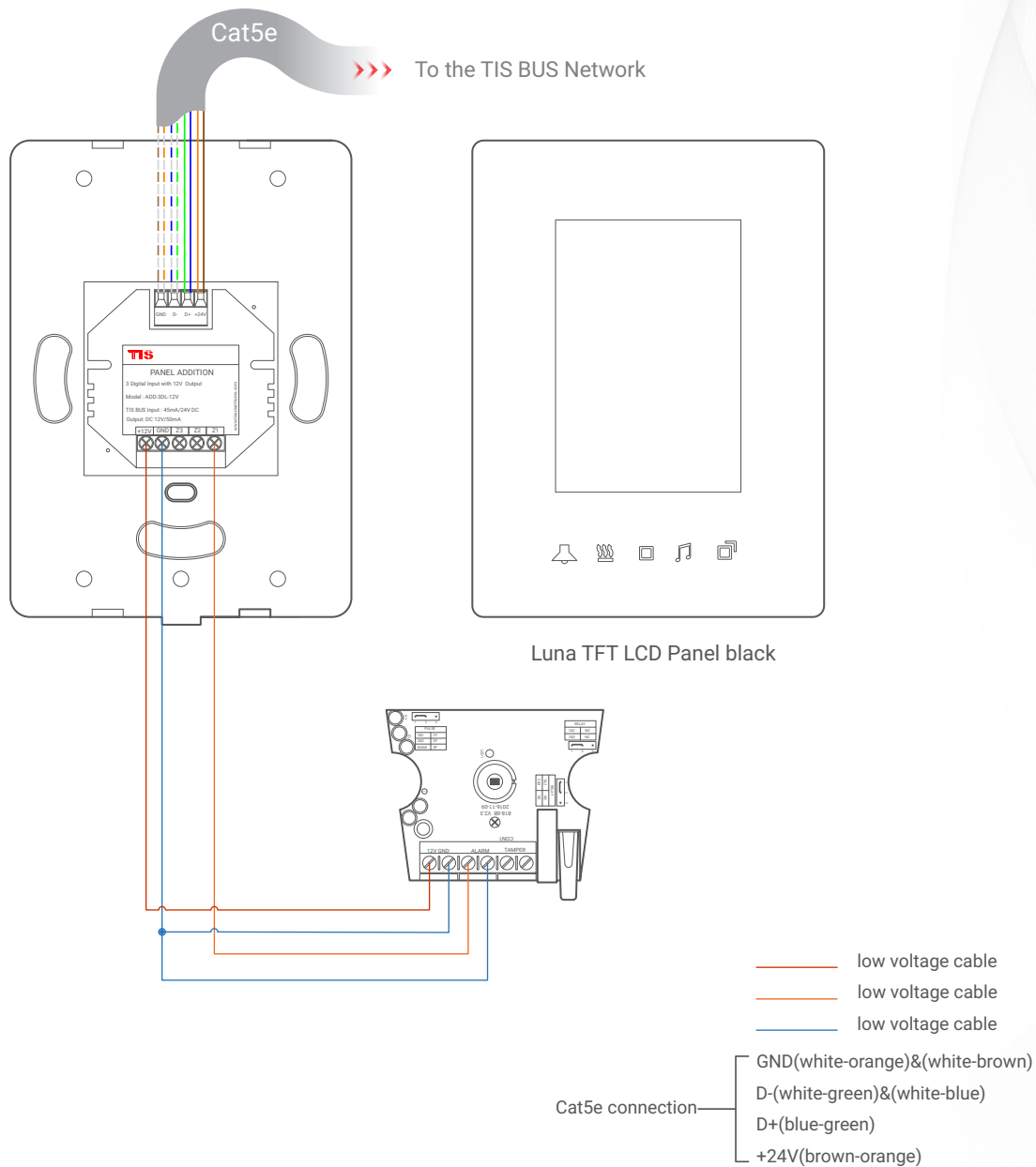
▲ Figure 6: Luna TFT & ADD-3DL-12V 3 rd Party Sensor Connection Diagram
