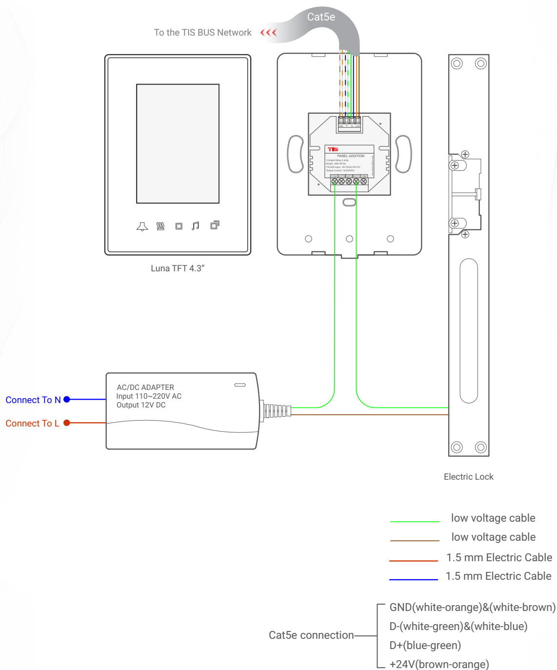
▲ Figure 4: Luna TFT & ADD-3R-5A Electric Lock Connection Diagram
