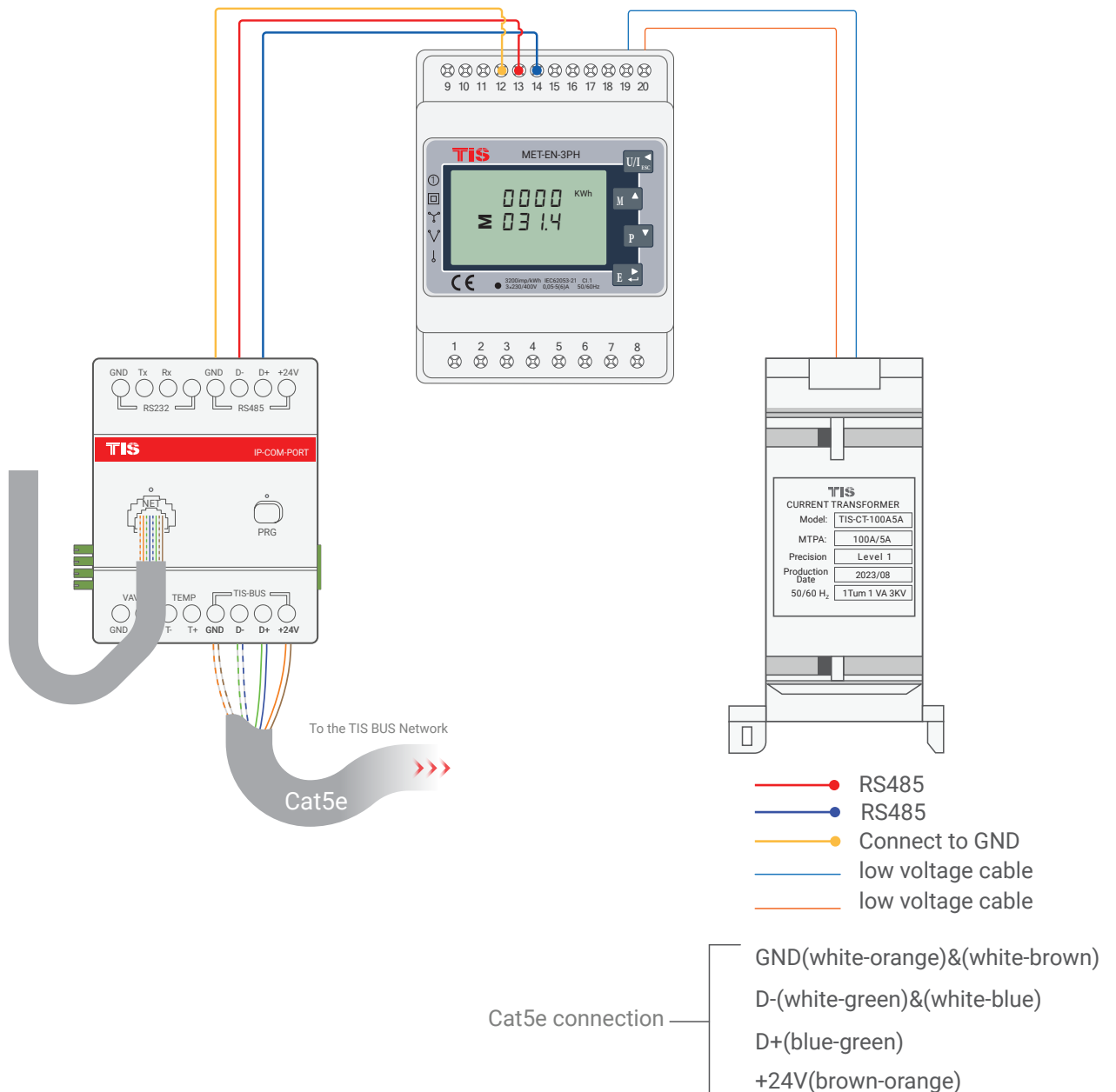
▲ Current Transformer and RS485 Connection Diagram
