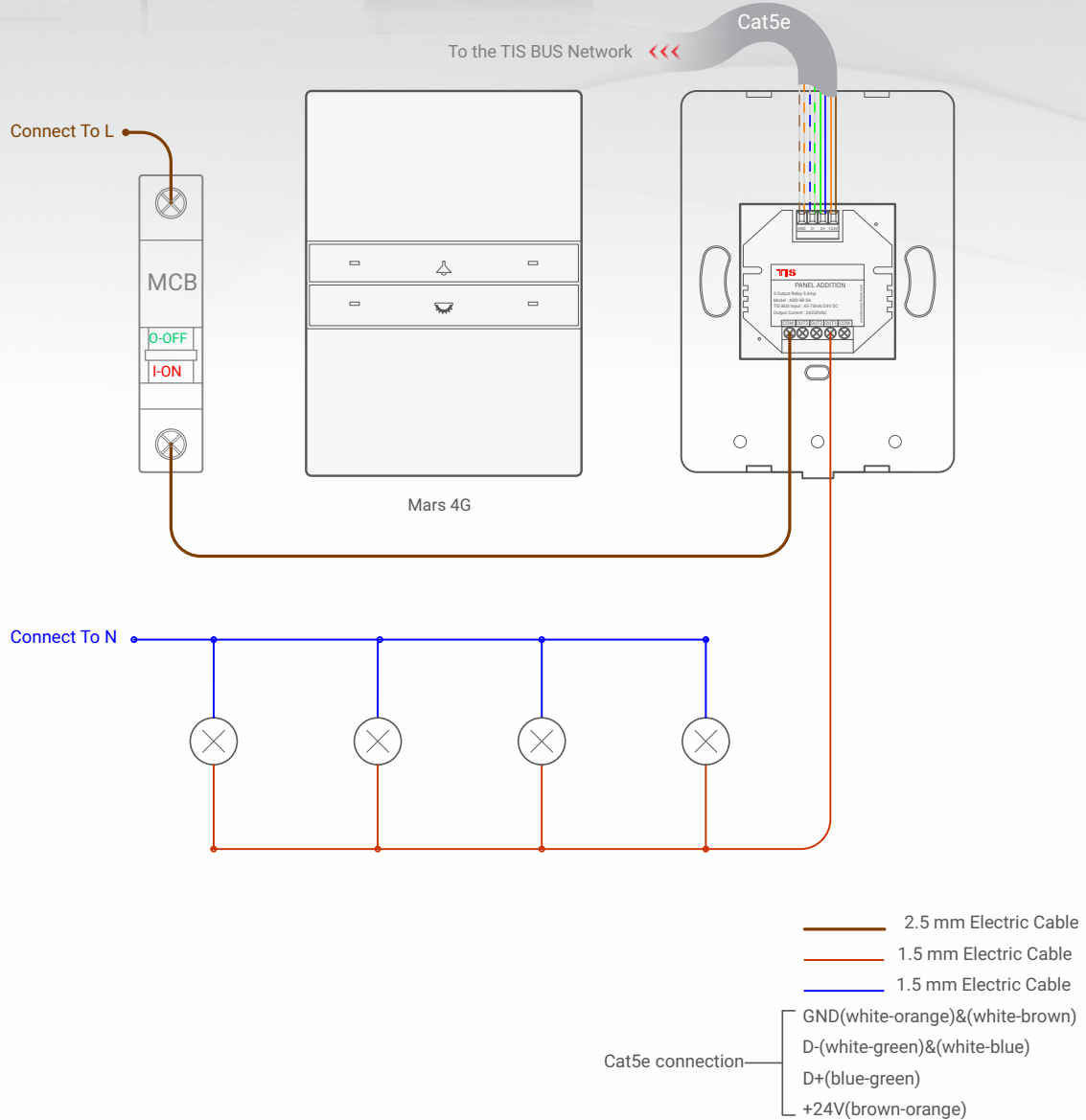
▲ Figure 1: Mars 4G & ADD-3R-5A Lights Connection Diagram
