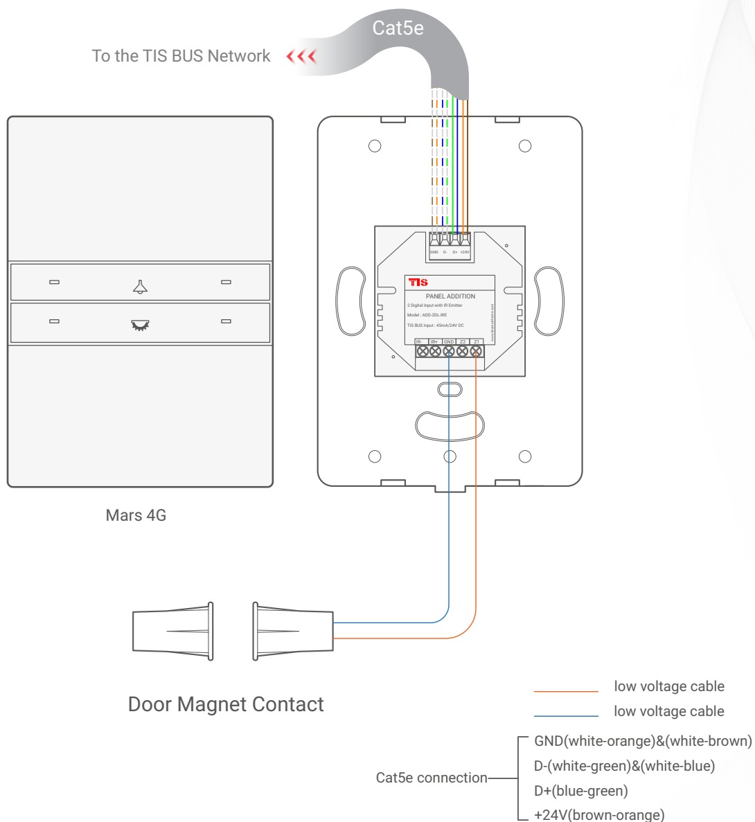
▲ Figure 11: Mars 4G & ADD-2DL-IRE Magnetic Door Contact Connection Diagram
