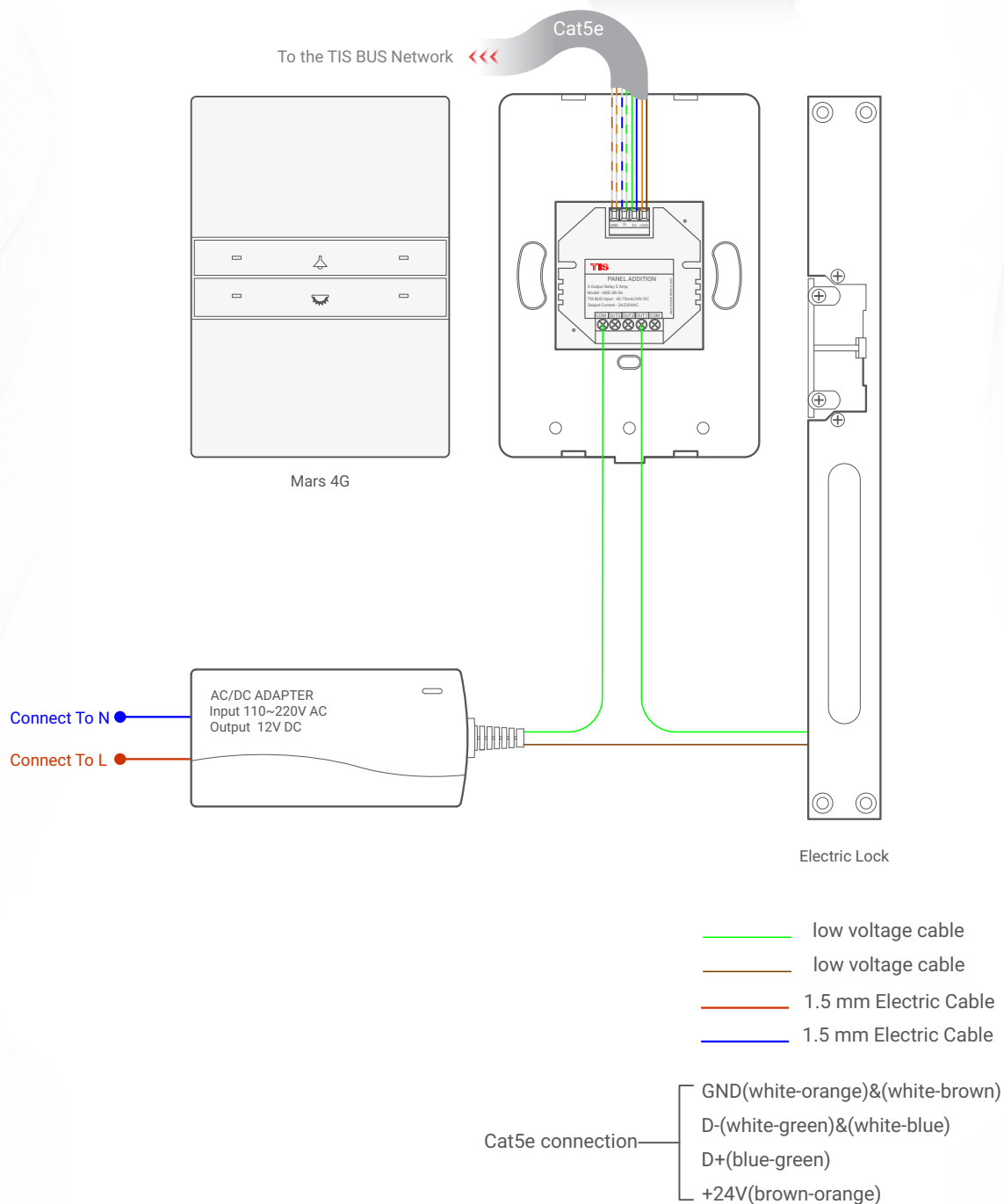
▲ Figure 4: Mars 4G & ADD-3R-5A Electric Lock Connection Diagram
