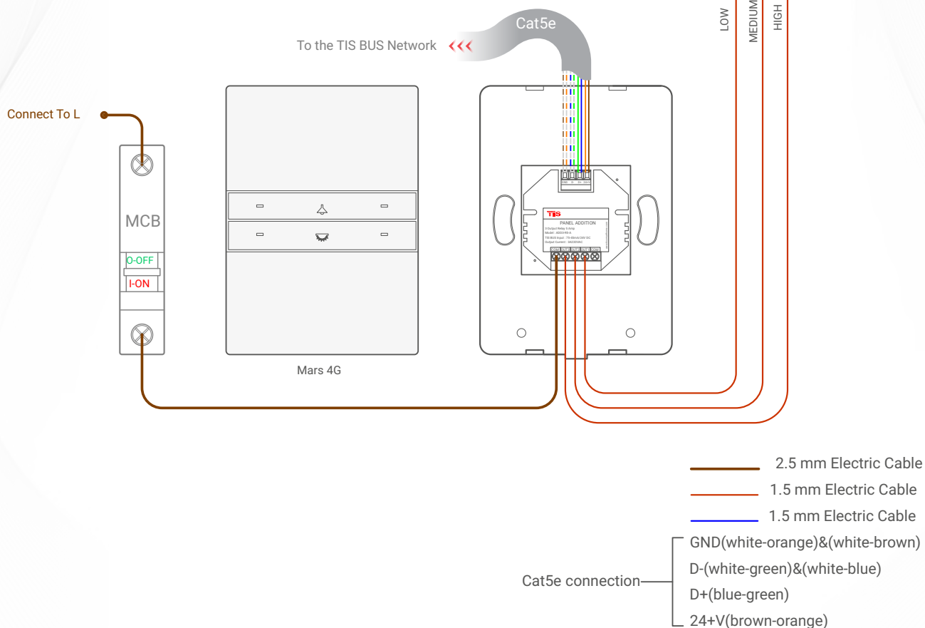
▲ Figure 2: Mars 4G & ADD-3R-5A FCU Connection Diagram
