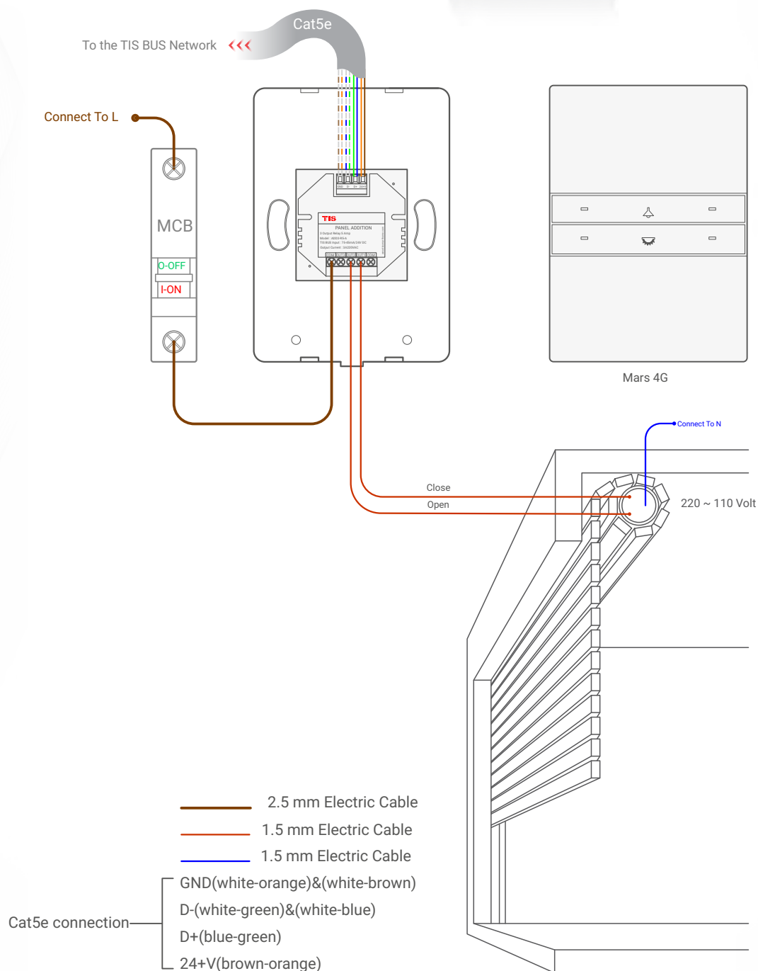
▲ Figure 3: Mars 4G & ADD-3R-5A Motors Connection Diagram
