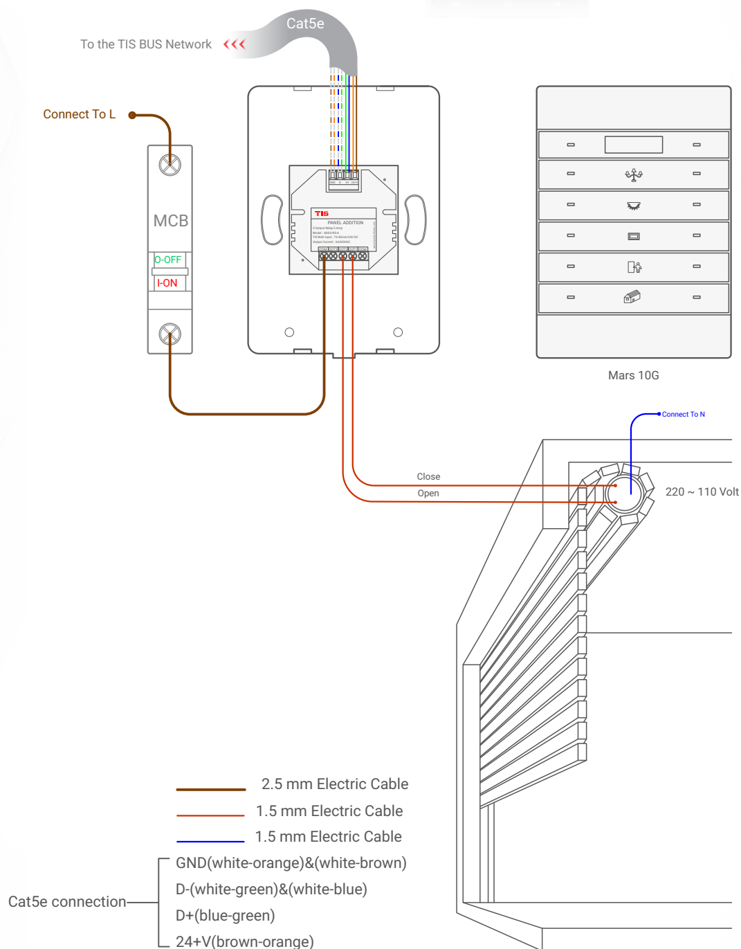
▲ Figure 3: Mars 10G & ADD-3R-5A Motors Connection Diagram
