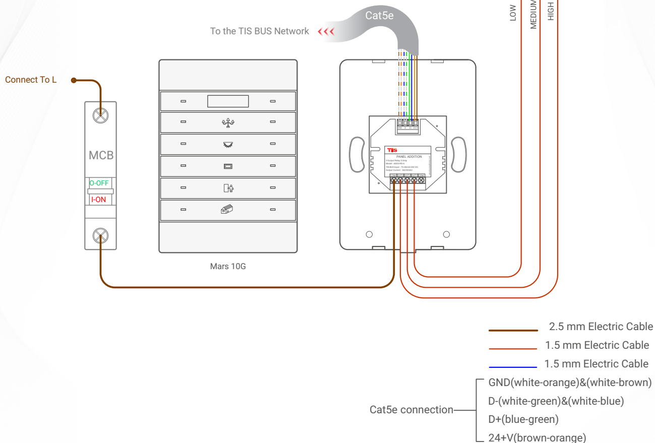
▲ Figure 2: Mars 10G & ADD-3R-5A FCU Connection Diagram
