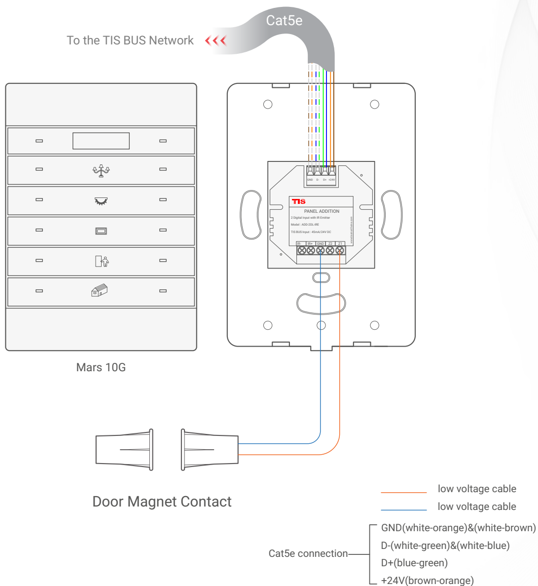
▲ Figure 11: Mars 10G & ADD-2DL-IRE Magnetic Door Contact Connection Diagram
