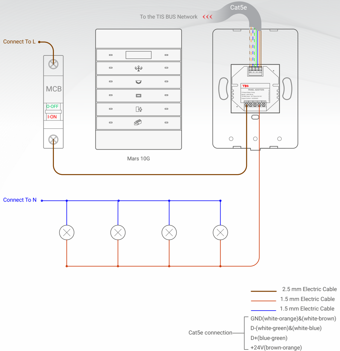
▲ Figure 1: Mars 10G & ADD-3R-5A Lights Connection Diagram
