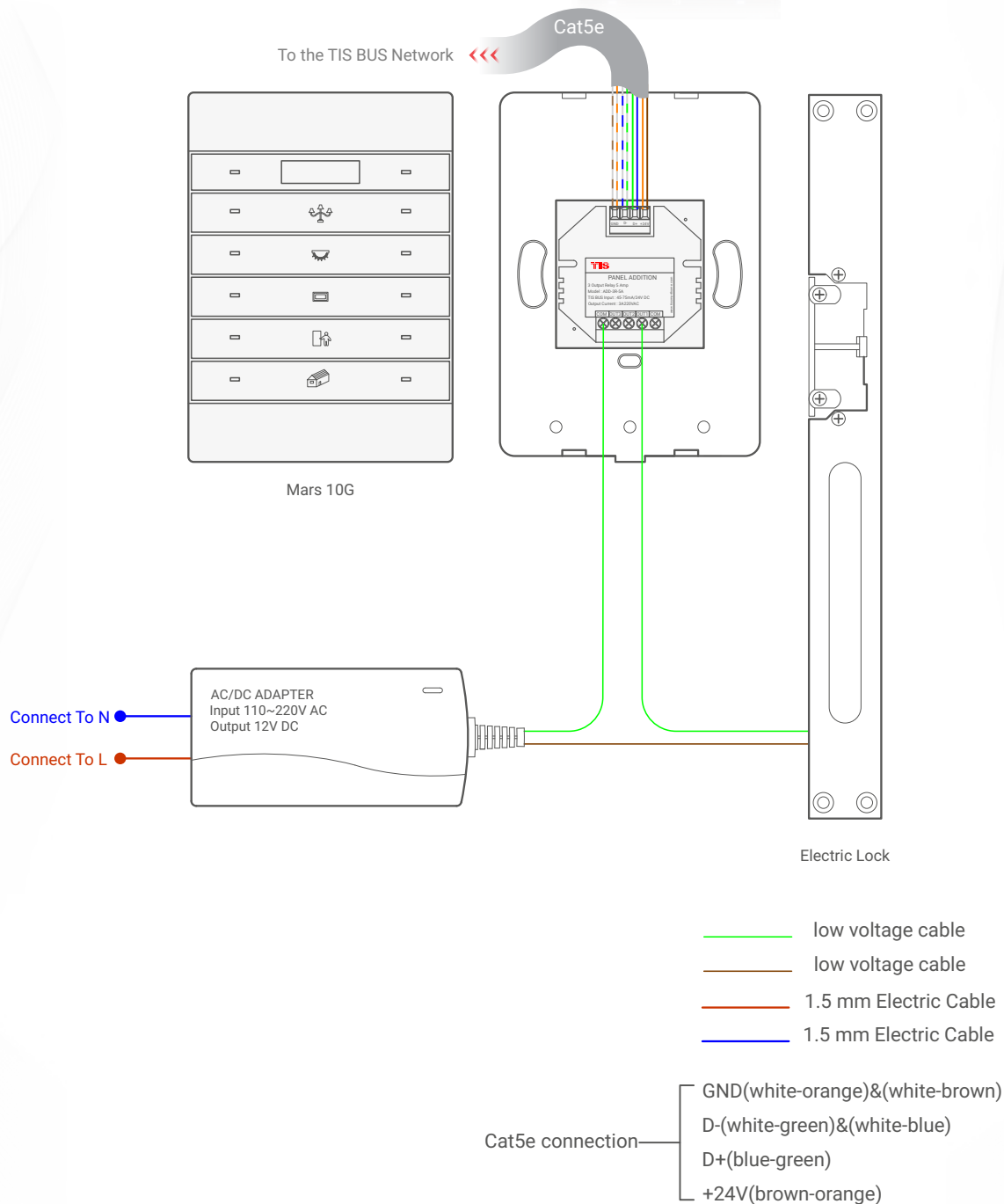
▲ Figure 4: Mars 10G & ADD-3R-5A Electric Lock Connection Diagram
