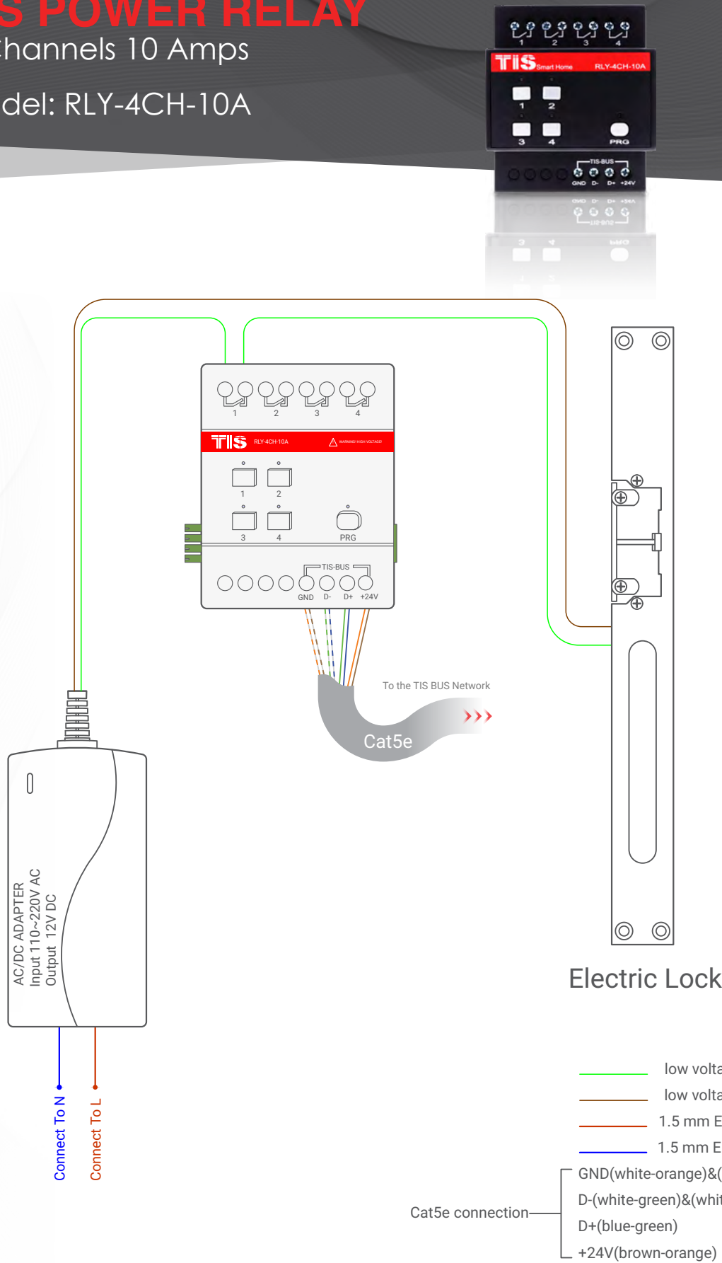
▲ Figure 3: Electric Lock Connection Diagram
