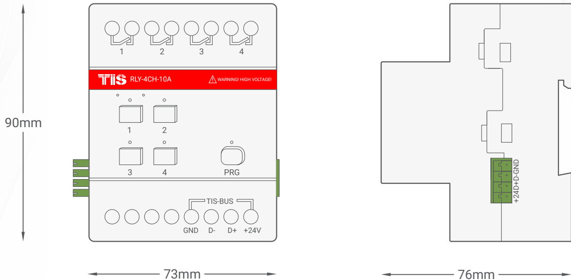
▲ Figure 6: Module's Dimension Diagram
