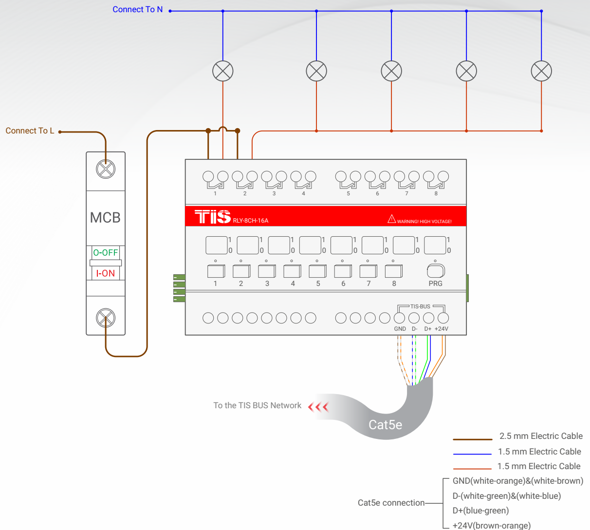
▲ Figure 1: Lights Connection Diagram
