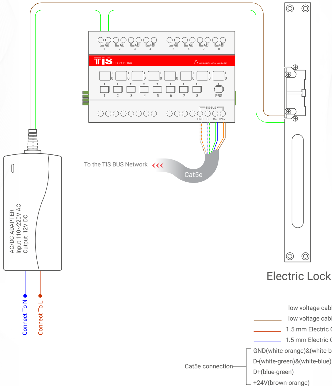
▲ Figure 3: Electric Lock Connection Diagram
