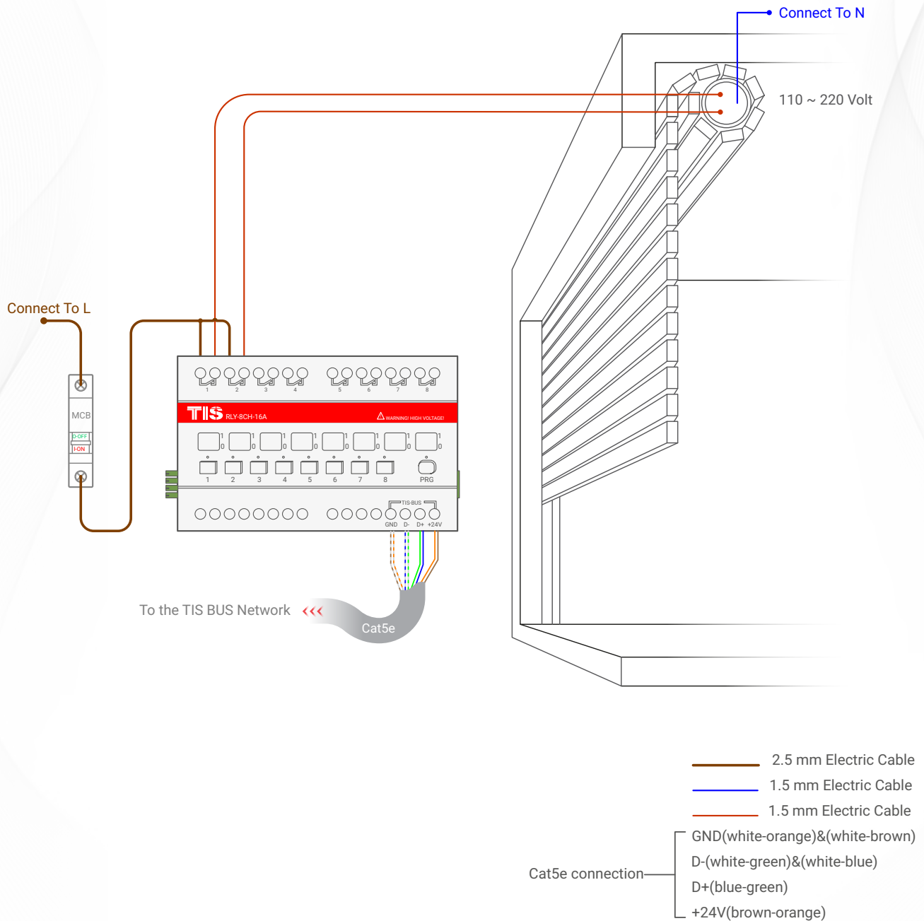
▲ Figure 2: Motors Connection Diagram
