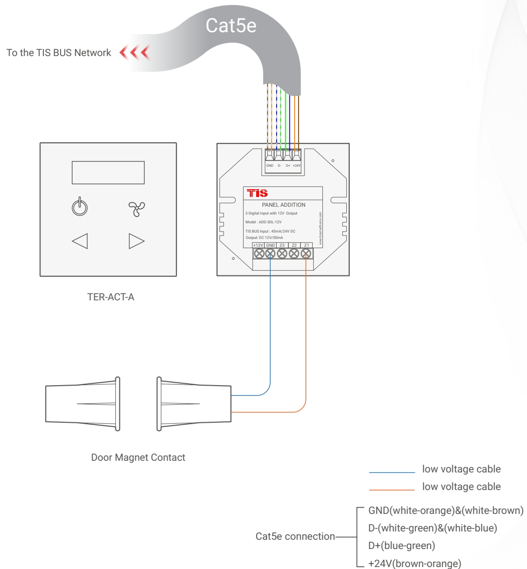
▲ Figure 5: TER-ACT-A & ADD-3DL-12V Magnetic Door Contact Connection Diagram
