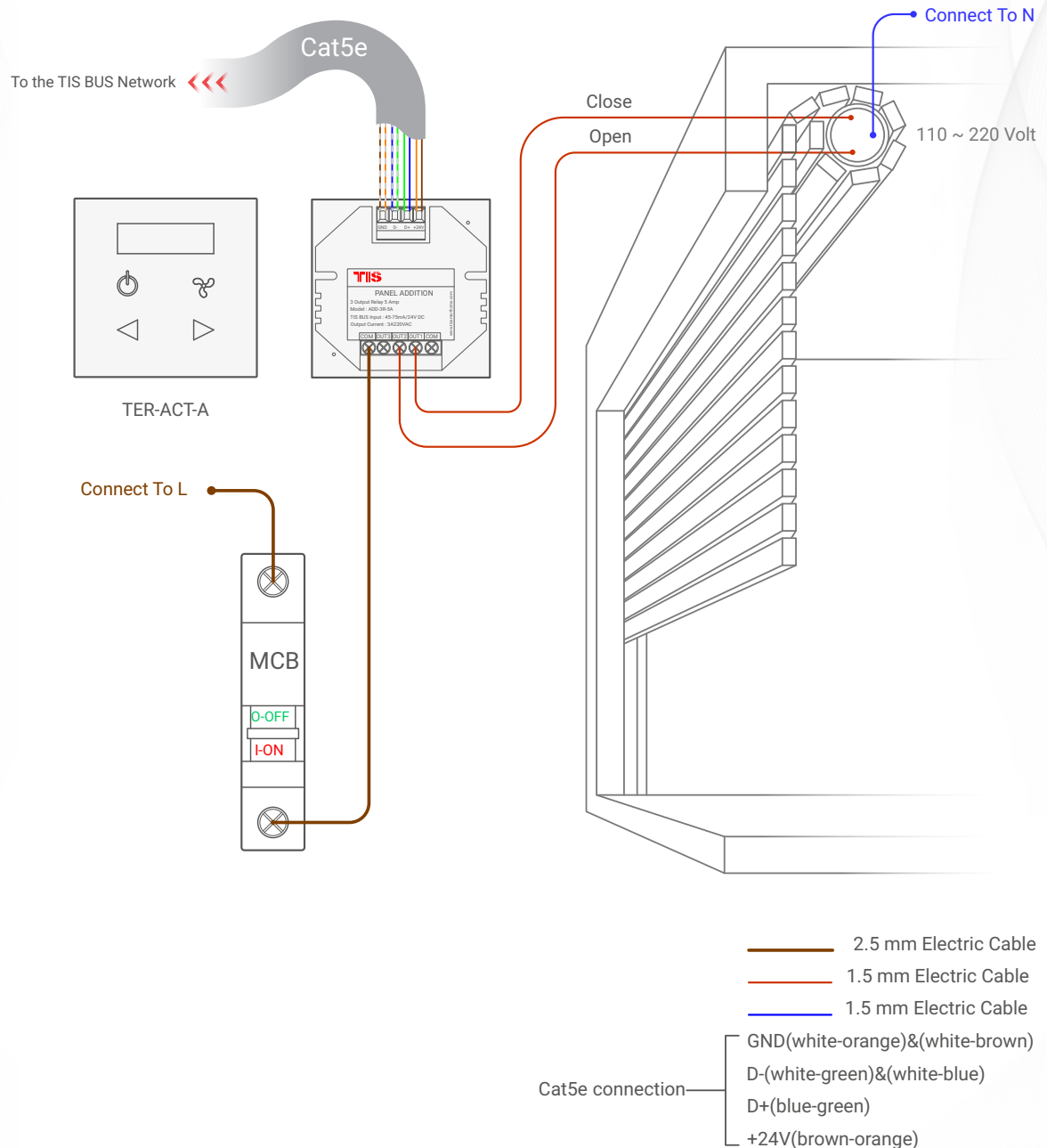
▲ Figure 2: TER-ACT-A & ADD-3R-5A Motors Connection Diagram
