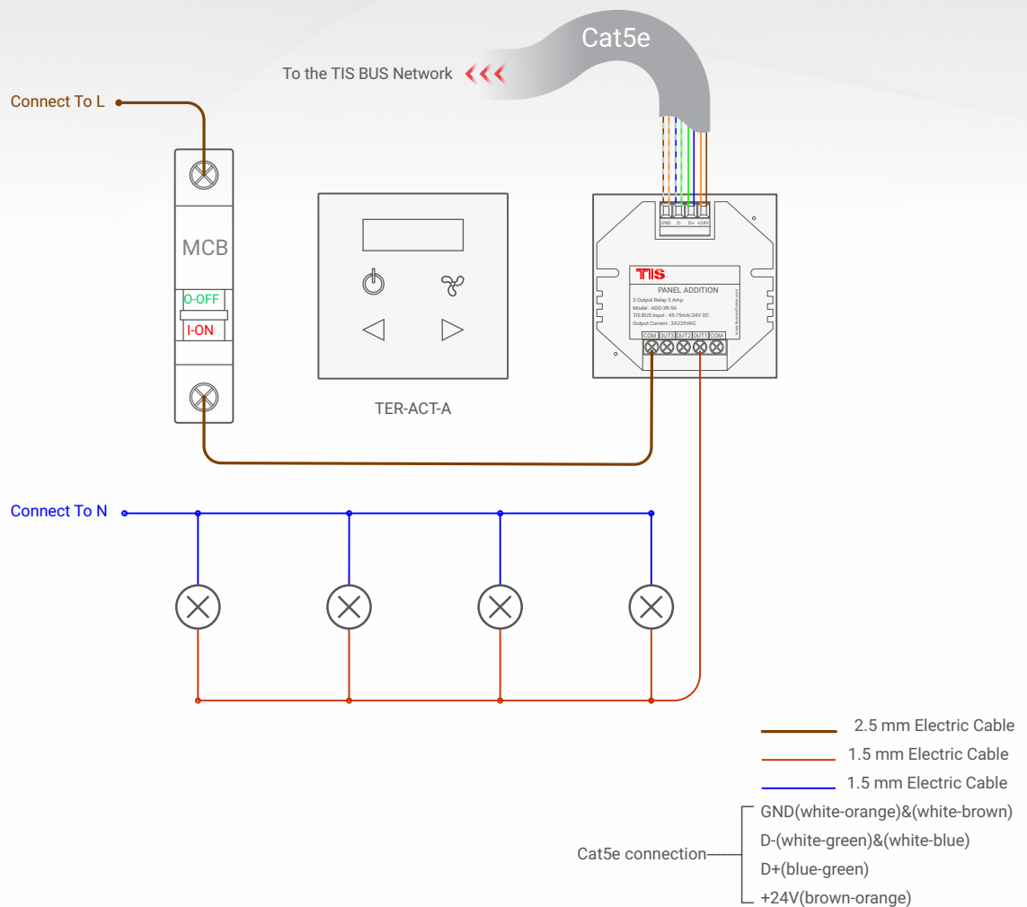
▲ Figure 1: TER-ACT-A & ADD-3R-5A Lights Connection Diagram
