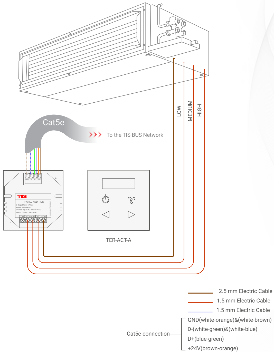
▲ Figure 3: TER-ACT-A & ADD-3R-5A FCU Connection Diagram
