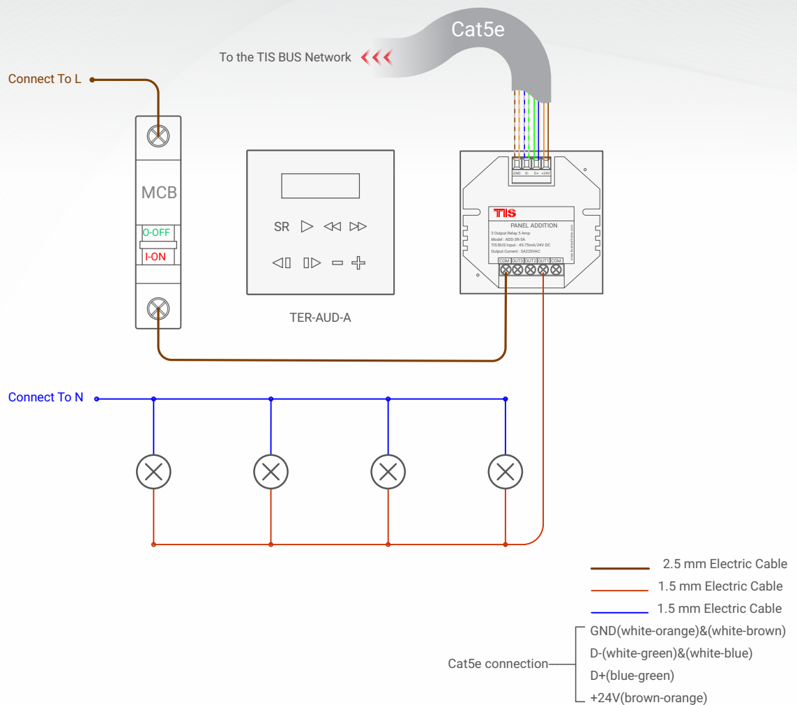
▲ Figure 1: TER-AUD-A & ADD-3R-5A Lights Connection Diagram
