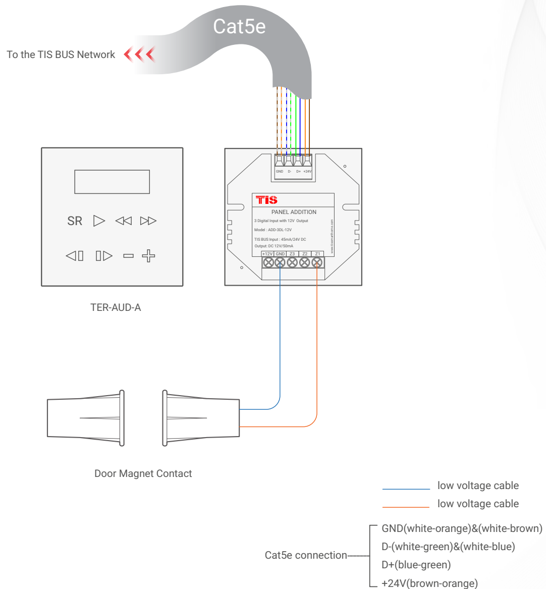
▲ Figure 5: TER-AUD-A & ADD-3DL-12V Magnetic Door Contact Connection Diagram
