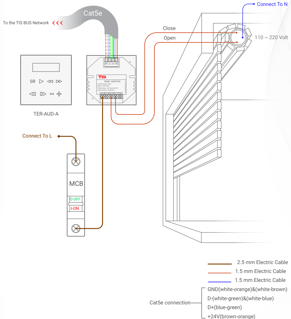
▲ Figure 2: TER-AUD-A & ADD-3R-5A Motors Connection Diagram
