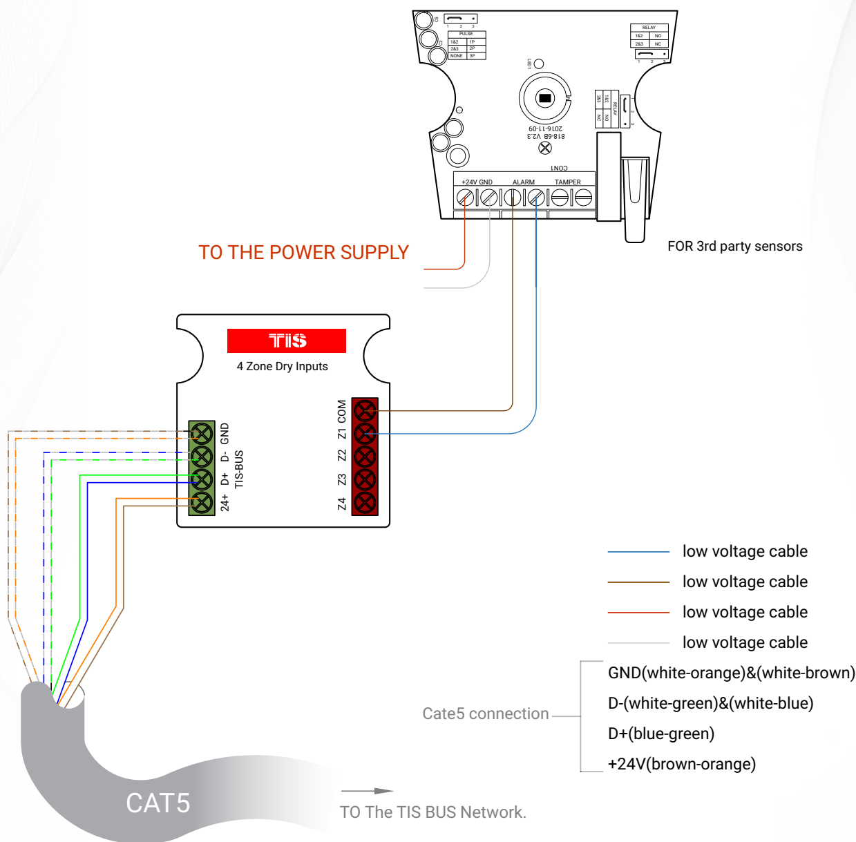
▲ Figure 3: 3 rd Party Sensor Connection Diagram
