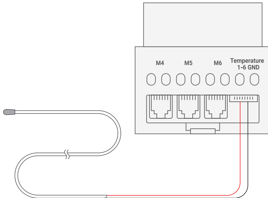
TIS Temp Sensor Probe
