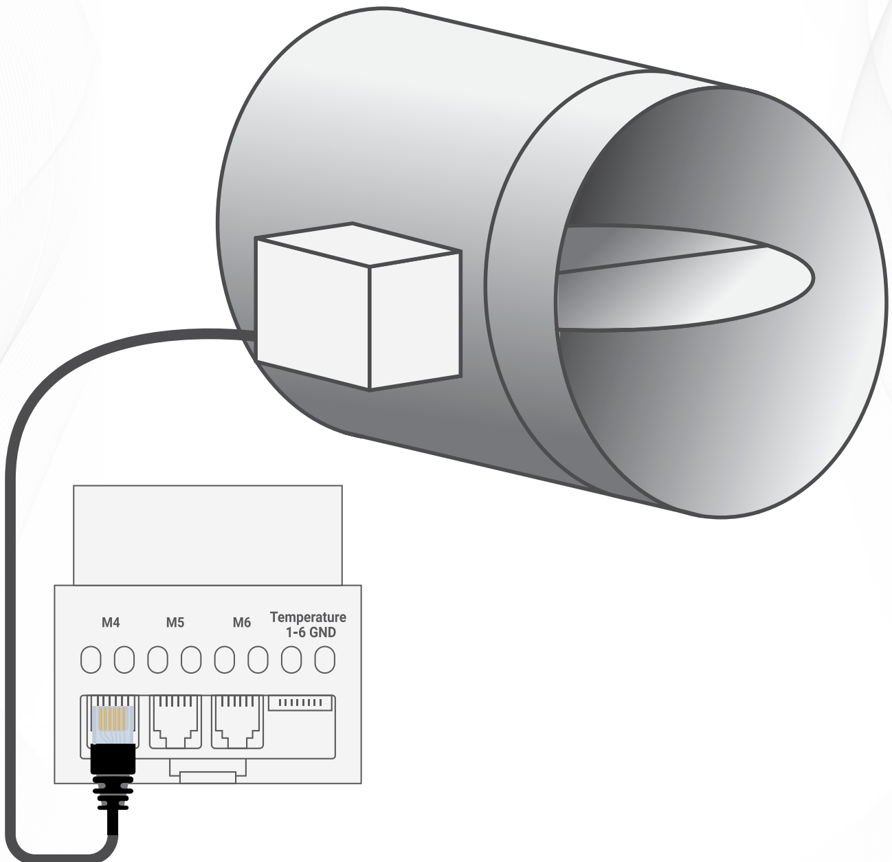
▲ TIS AC Zoning Module & Motorized Air Damper Diagram
