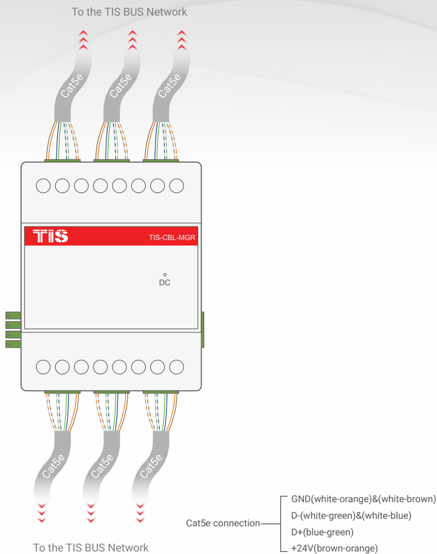
▲ Figure 1: Module's BUS Connection Diagram
