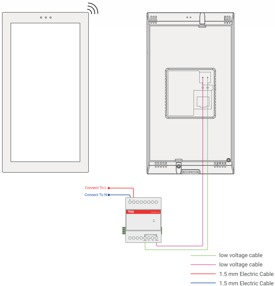
▲ Saturn switch connection with power supply connection diagram (Connect to TIS-BUS network via WiFi)
