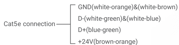
▲ Figure 7: TIT-4G-BUS-K-3R Module's Bus Connection Color Coding
