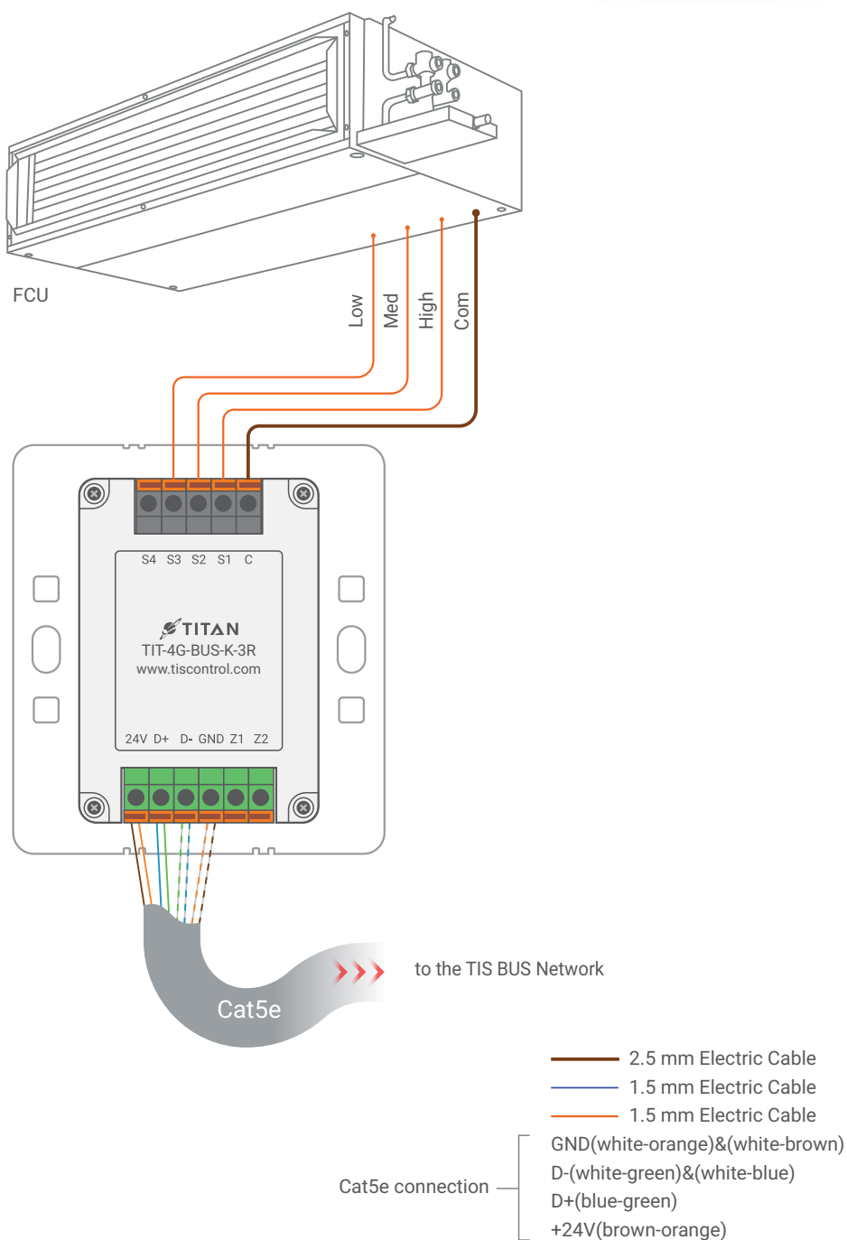
▲ Figure 2: TIT-4G-BUS-K-3R & FCU Connection Diagram
