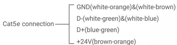
▲ Figure 7: TIT-4G-BUS-S-3R Module's Bus Connection Color Coding
