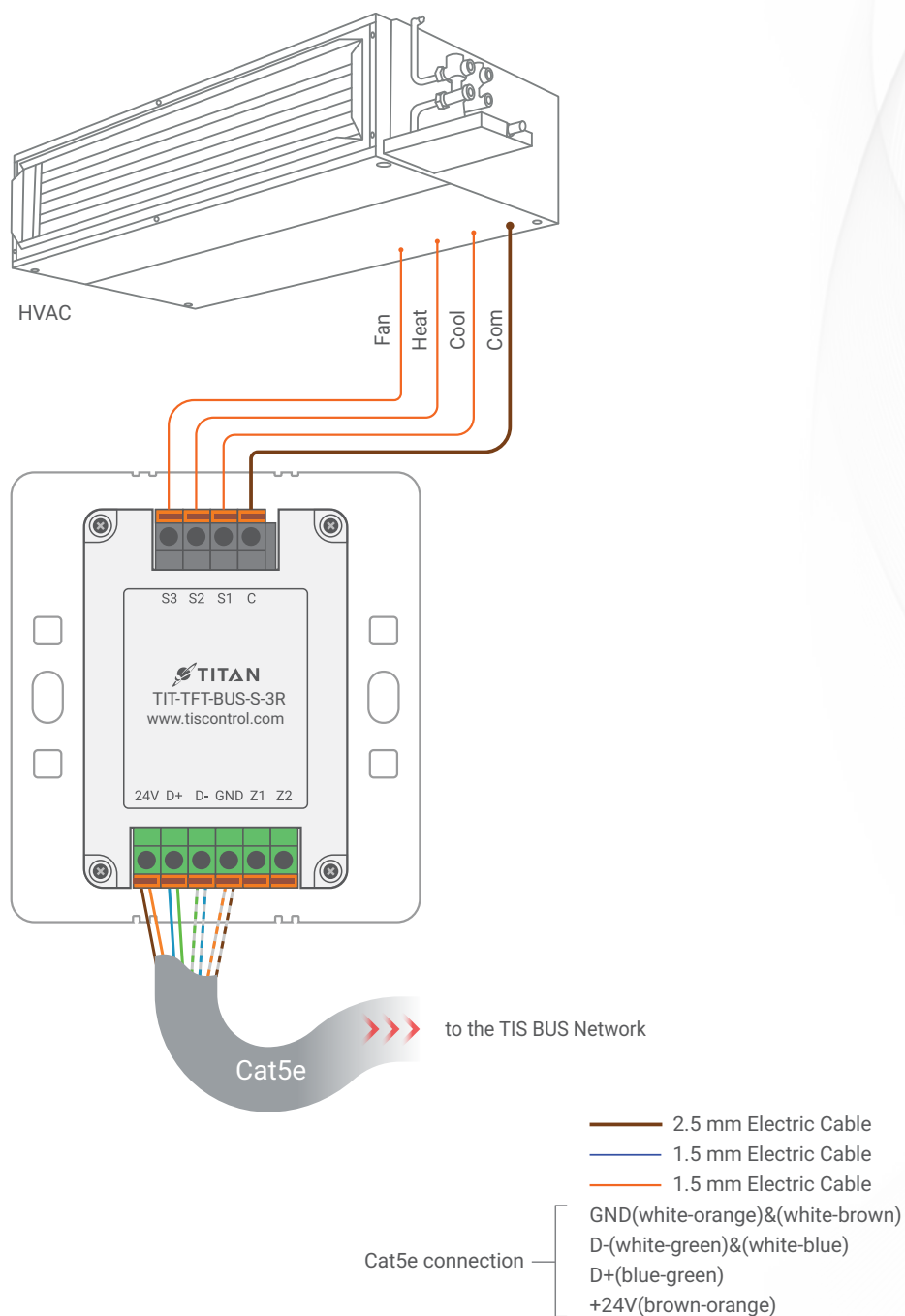
▲ Figure 3: TIT-TFT-BUS-S-3R & HVAC Connection Diagram
