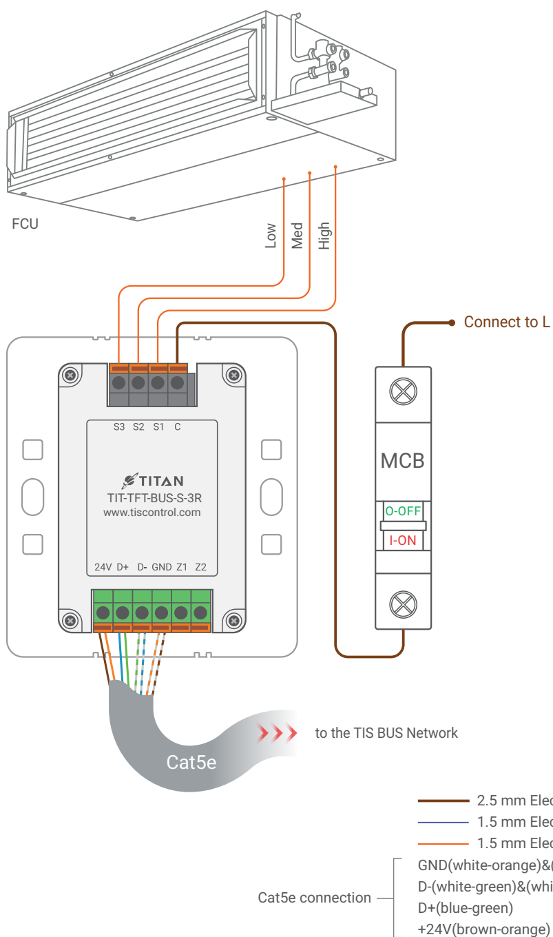
▲ Figure 2: TIT-TFT-BUS-S-3R & FCU Connection Diagram
