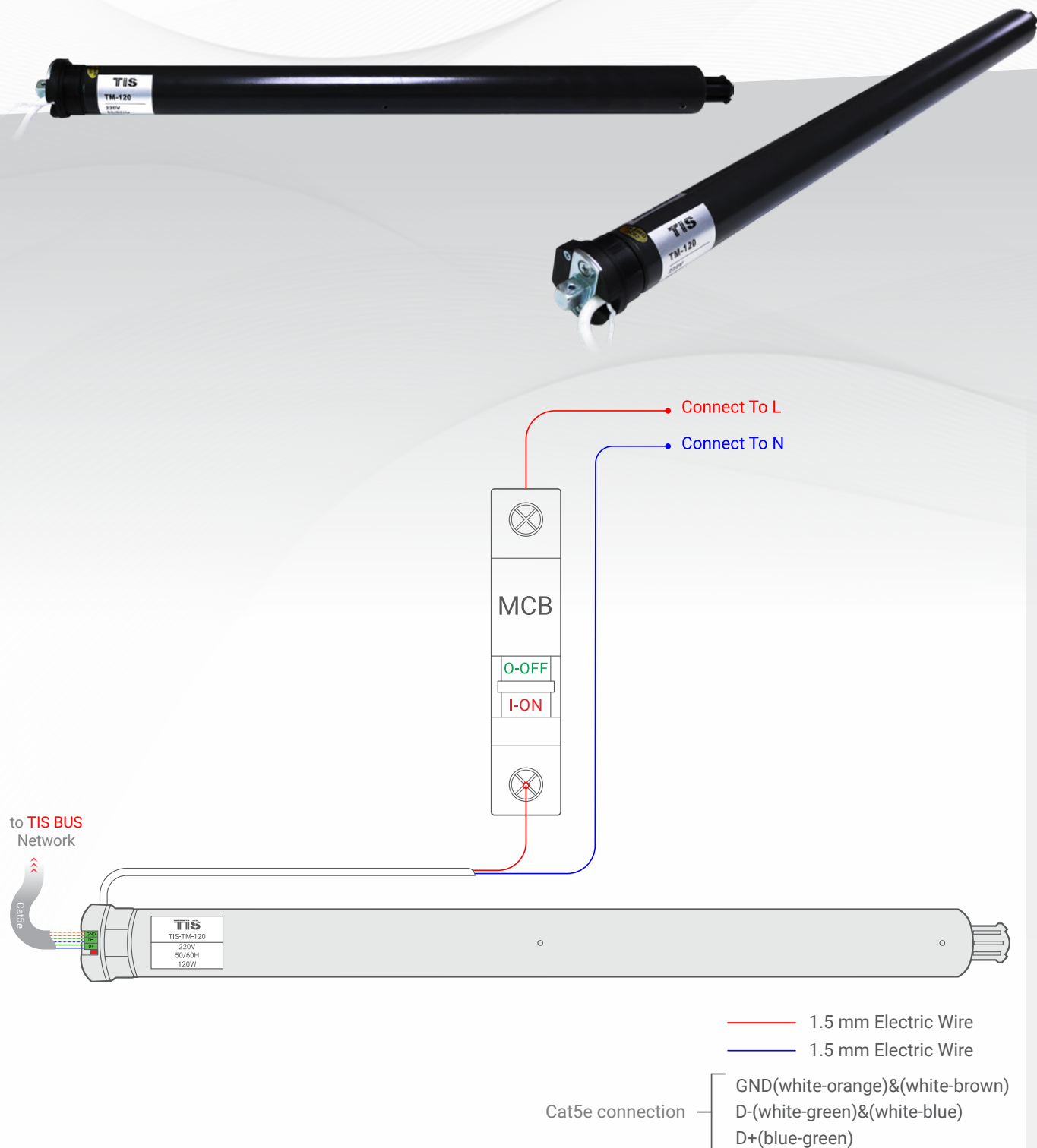
▲ Figure 1: Roller Curtain Motor's Bus Connection Diagram
