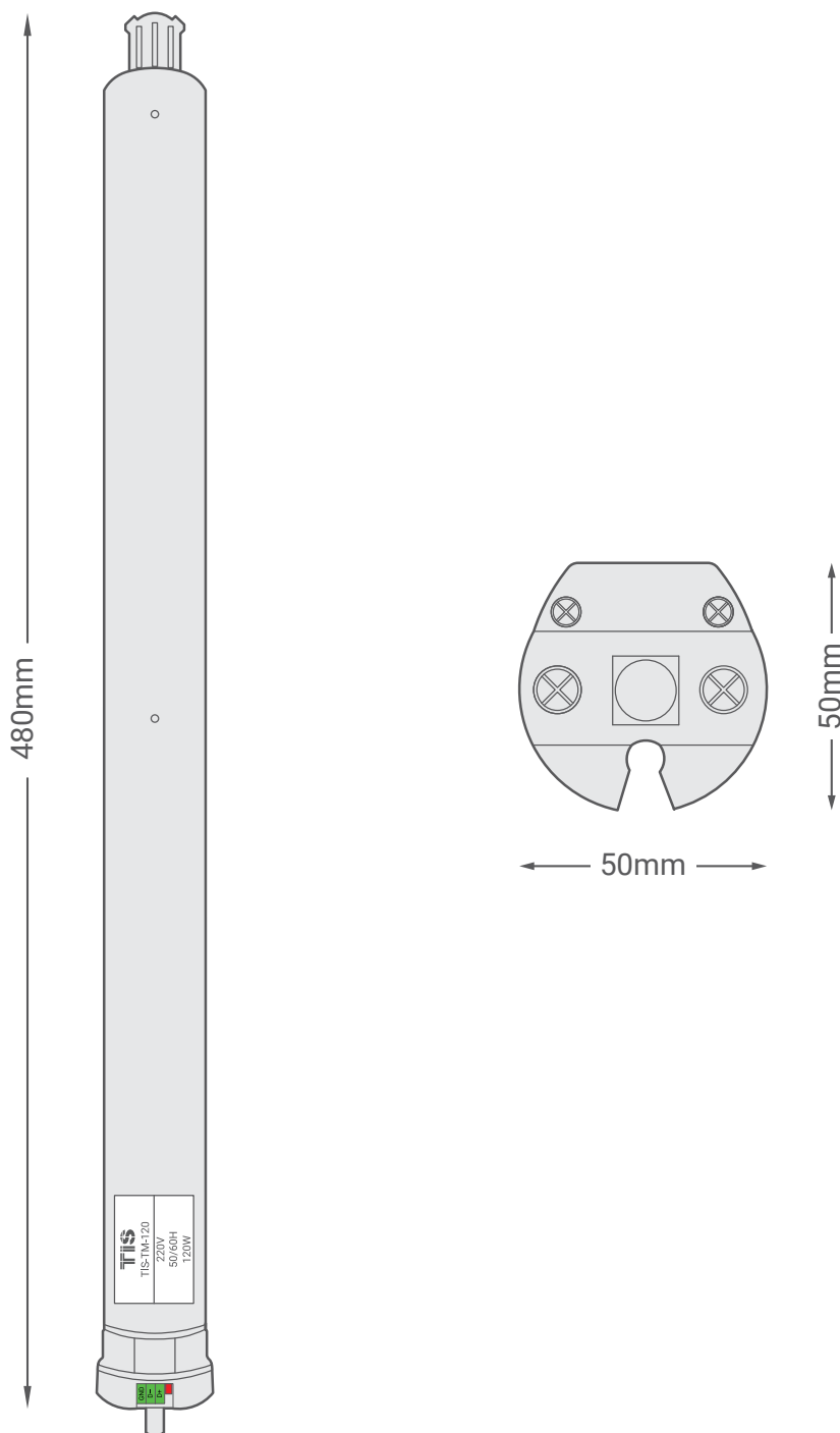
▲ Figure 3: Module Dimensions
