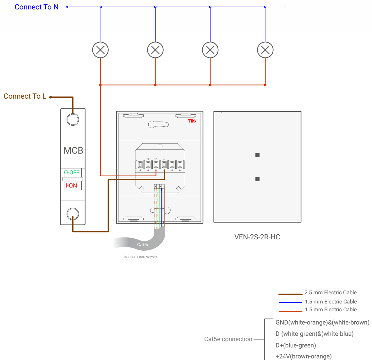
▲ Figure 1: VEN-2S-2R-HC Lights Connection Diagram
