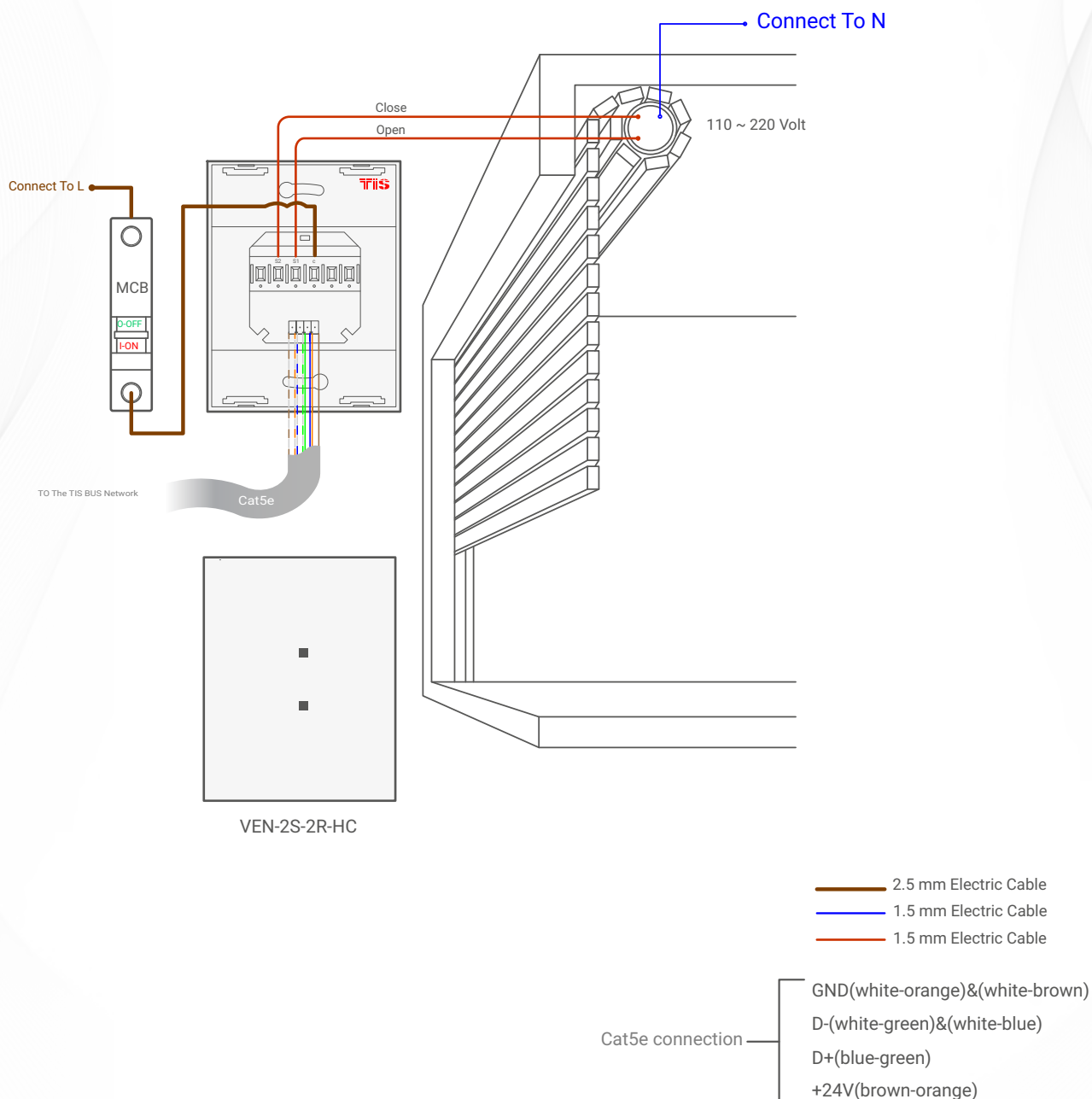
▲ Figure 2: VEN-2S-2R-HC & Motors Connection Diagram
