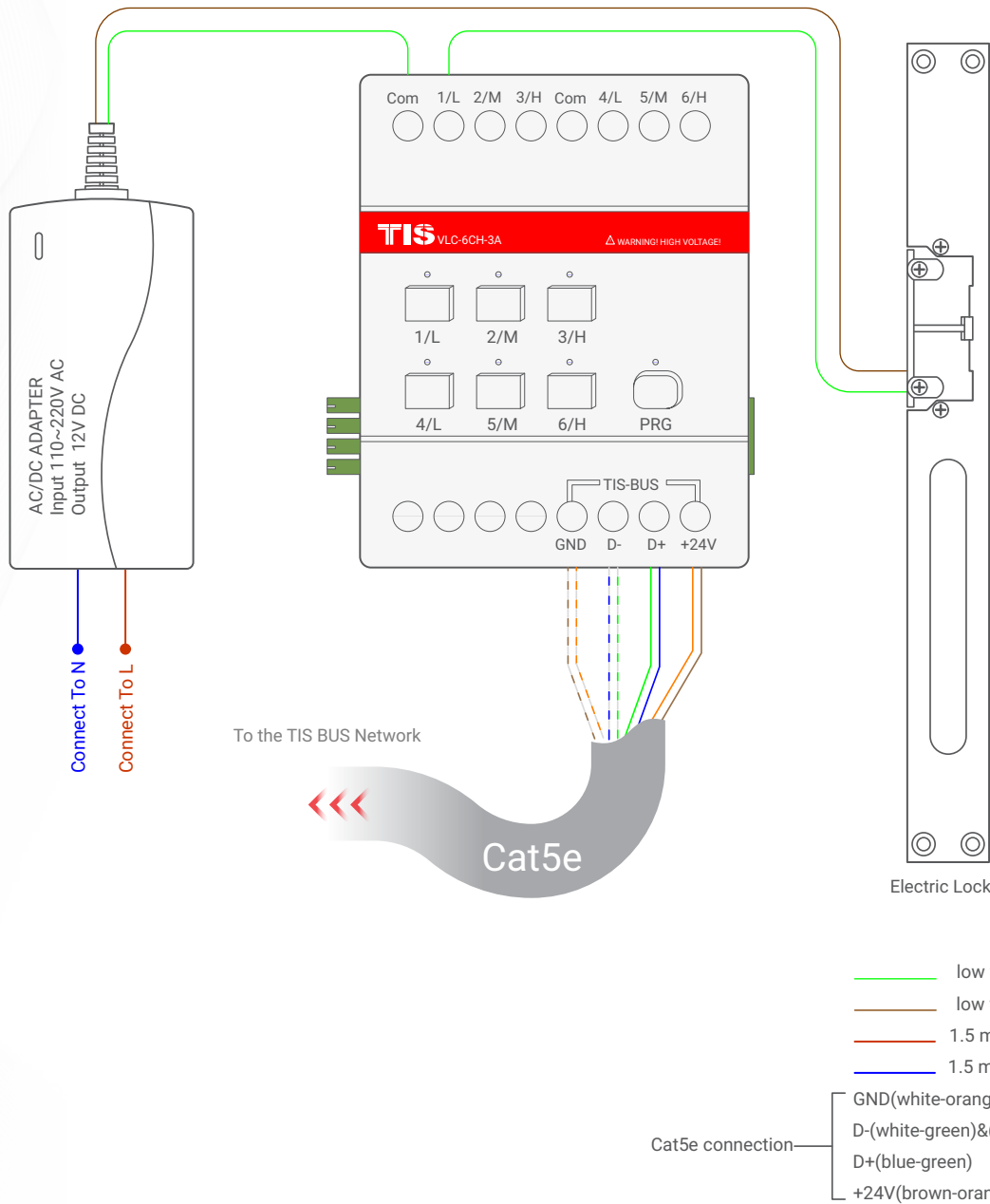
▲ Figure 4: Electric Lock Connection Diagram
